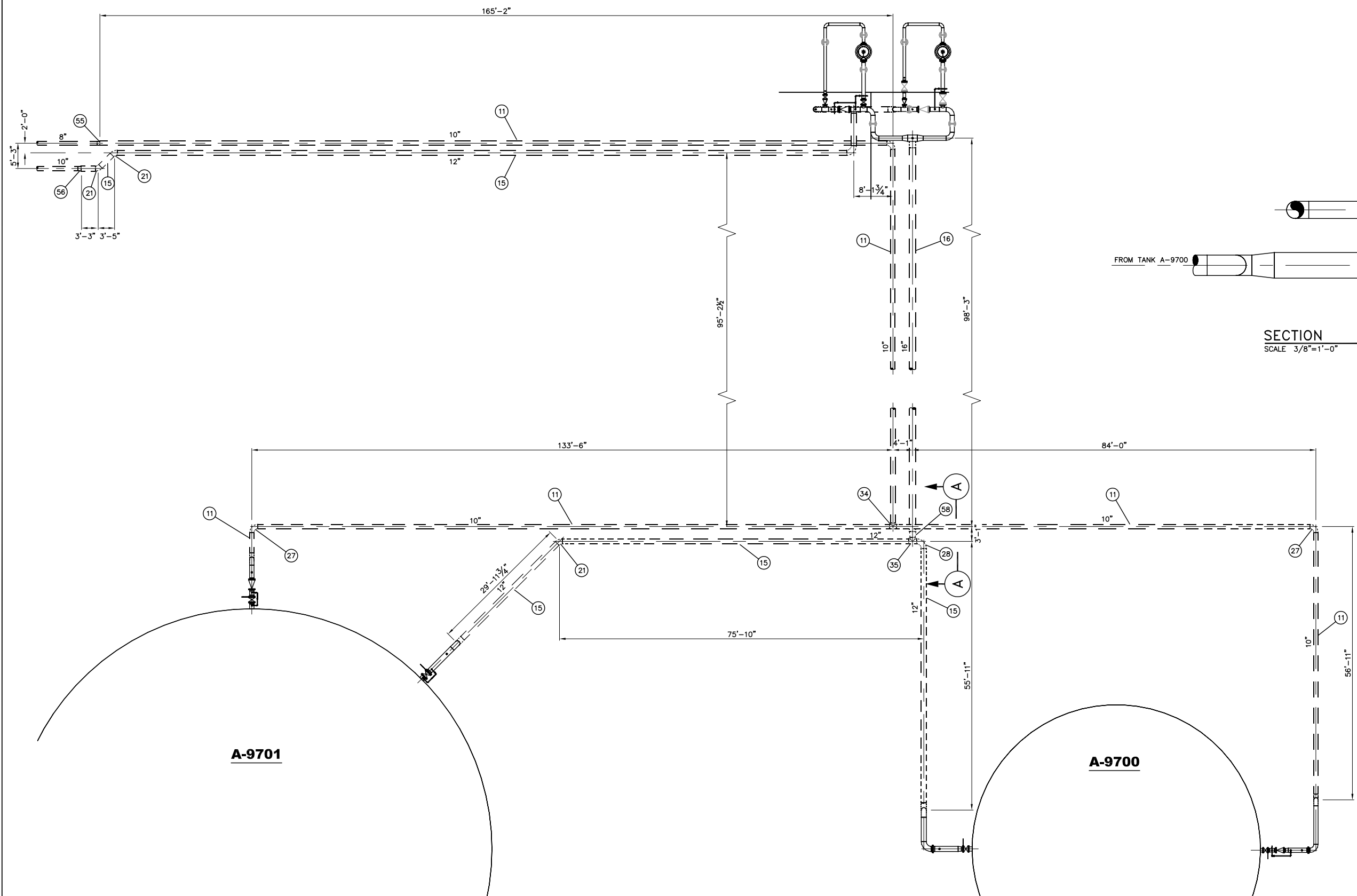
PLAN SCALE 1/8"=1'-0"
