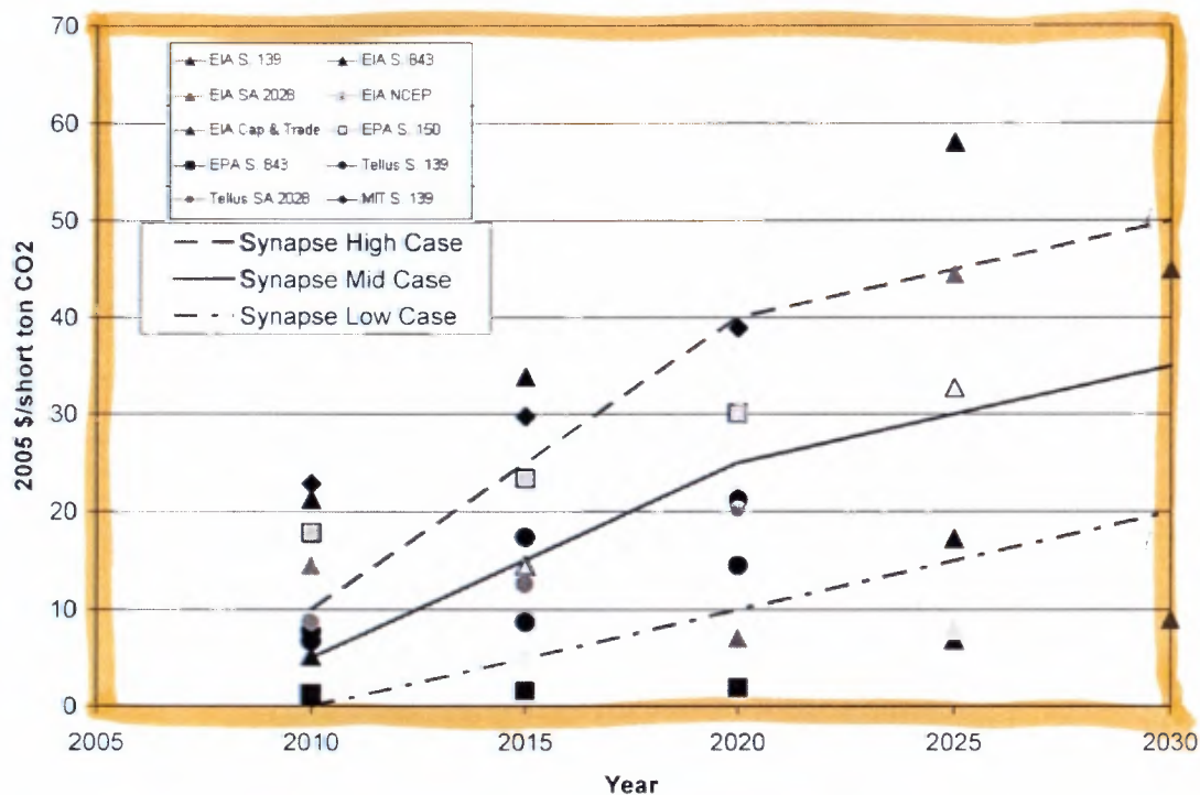
1 Figure 2. Synapse Carbon Dioxide Prices
