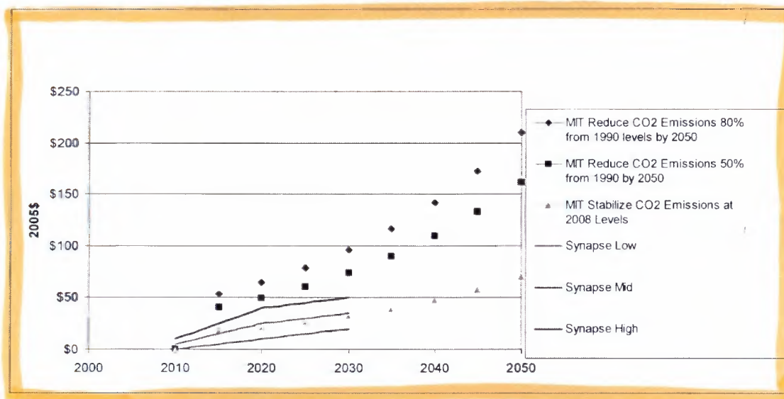
1 Figure 4: CO 2 Price Scenarios – Synapse and Core Scenarios in April 2 2007 MIT Assessment of U.S. Cap-and-Trade Proposals
