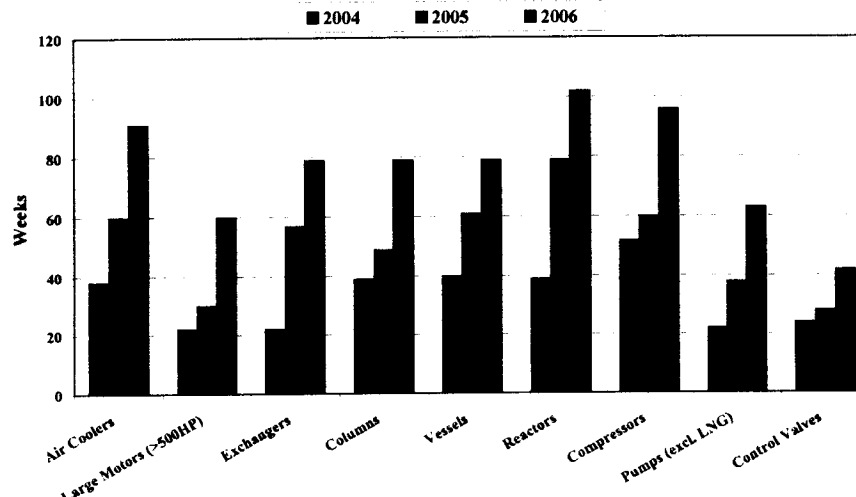
Figure 14 Delivery Schedules
