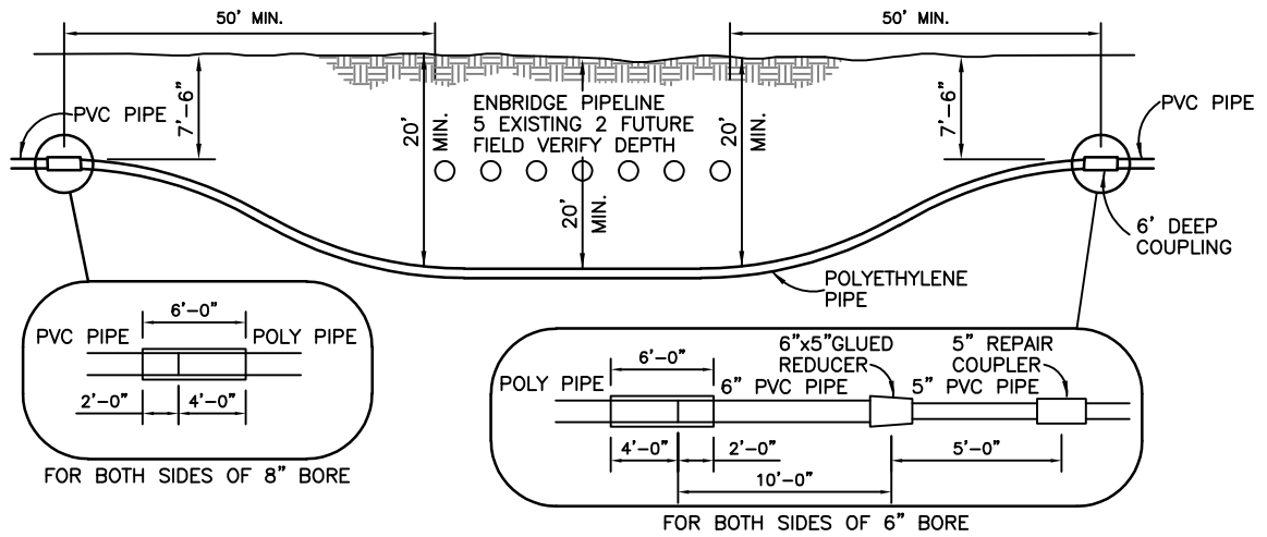
1 1 ENBRIDGE PIPELINE CROSSING DETAIL SCALE: NONE
