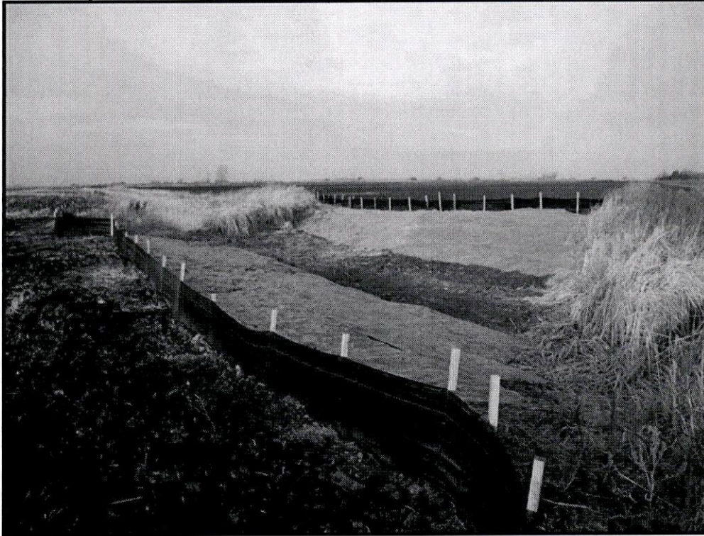
Restored right-of-way after decompaction and topsoil discing
