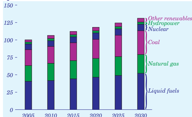
Figure 34. Primary energy use by fuel, 2005-2030 (quadrillion Btu)
