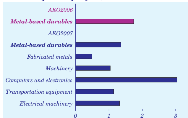
Figure 18. Average annual increases in energy demand for metal-based durables industries in the AEO2006 and AEO2007 reference case projections, 2005-2030 (percent per year)
