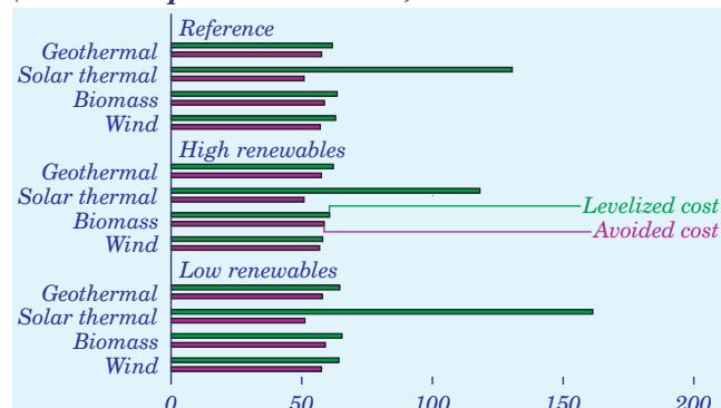
Figure 62. Levelized and avoided costs for new renewable plants in the Northwest, 2030 (2005 mills per kilowatthour)
