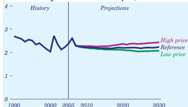
Figure 74. Average natural gas transmission and distribution margins, 1990-2030 (2005 dollars per thousand cubic feet)
