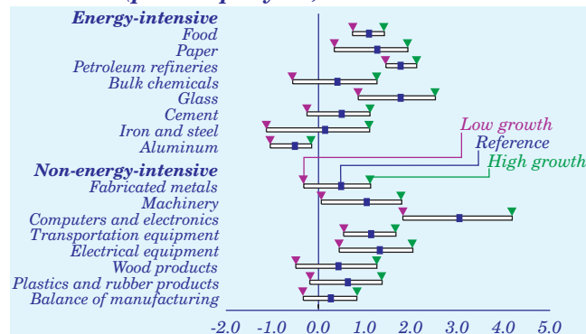
Figure 46. Average growth of delivered energy consumption in the manufacturing subsectors, 2005-2030 (percent per year)
