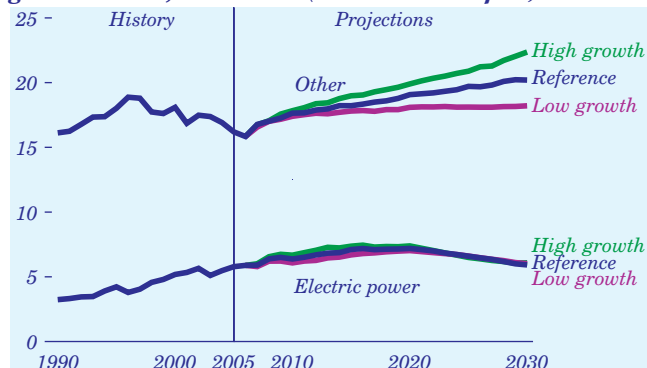
Figure 70. Natural gas consumption in the electric power and other end-use sectors in alternative growth cases, 1990-2030 (trillion cubic feet)
