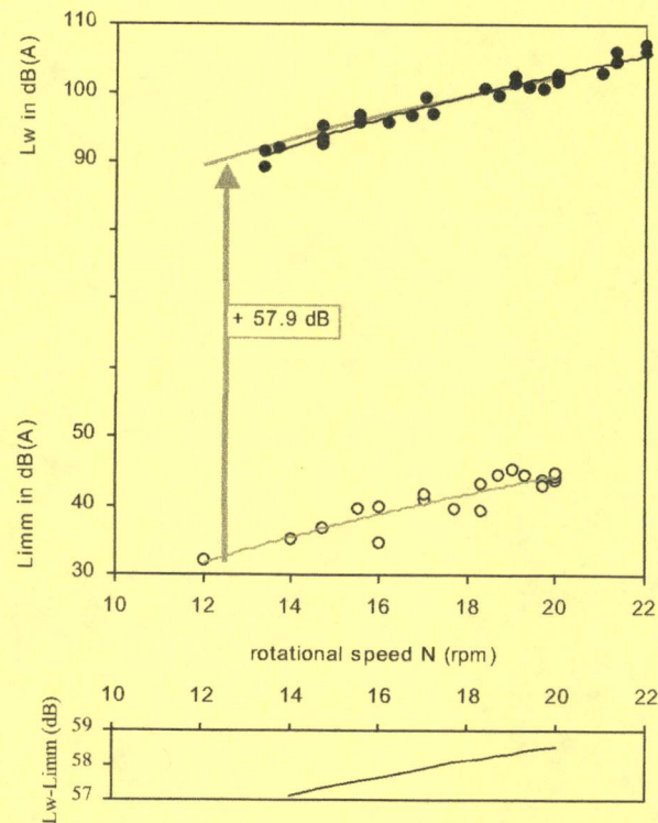
Fig. 7. Turbine sound power levels L_W measured near wind turbines ( \bullet ) and immission levels L_{imm} measured at 400 m from wind park ( \circ ): averages differ 57.9 dB; (below) increase of difference L_W - L_{imm} with rotational speed.
