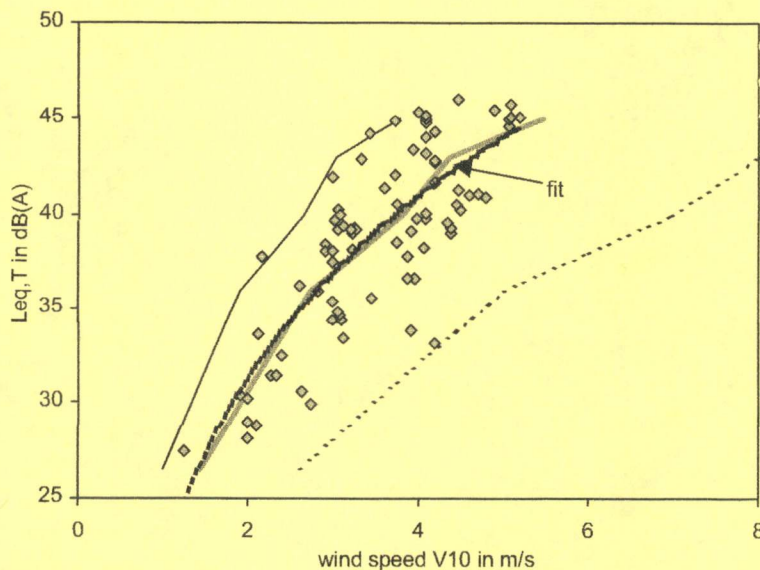
Fig. 6. Measured sound levels L_{eq,T} ( T = 20-60 min) at location A with best fit; and expected sound levels according to a logarithmic wind profile ( v_{98}/v_{10} = f_{log} = 1.4 ; dotted line), a stable wind profile ( v_{98}/v_{10} = 1.8 \cdot f_{log} ; thick grey line) and maximum wind speed ratio ( v_{98}/v_{10} = 2.6 \cdot f_{log} ; thin line).
