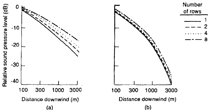
Figure 7-27. Calculated noise propagation downwind of various numbers of rows of wind turbines in the example array [Shepherd and Hubbard 1986]. (a) without atmospheric absorption. (b) \alpha = 0.54 dB/100 m.
