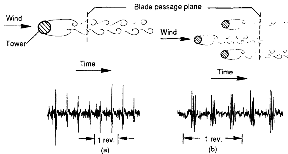
Figure 7-3. Sound pressure time histories from two downwind-rotor HAWTs [Shepherd, Willshire, and Hubbard 1988; Hubbard and Shepherd 1982]. (a) 78.2-m-diameter rotor, 2 blades, 2050-kW output, 30-rpm rotor speed, 200-m distance. (b) 17.6-m-diameter rotor, 3 blades, 5-kW output, 72-rpm rotor speed, 30.5-m distance.
