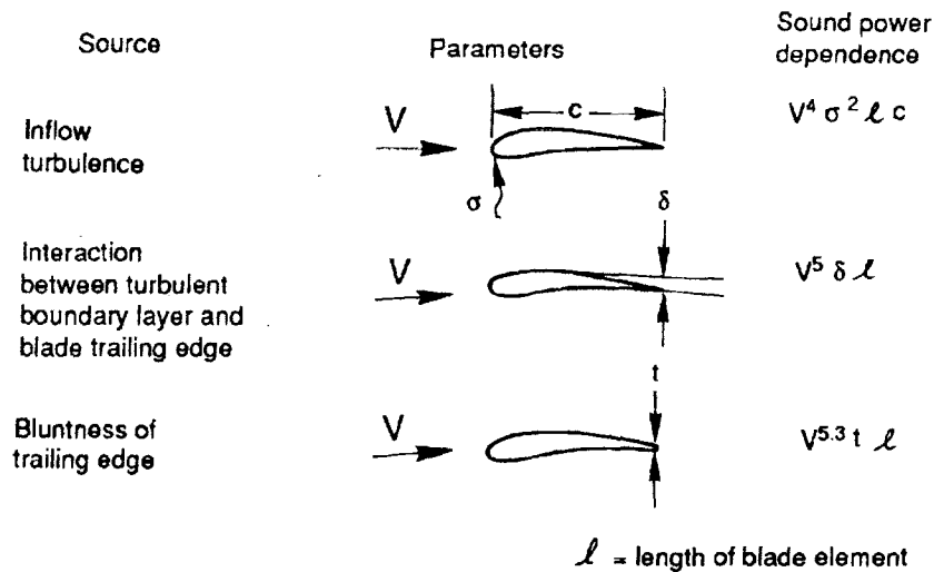
Figure 7-14. Sources of wind turbine broadband noise [Grosveld 1985]
