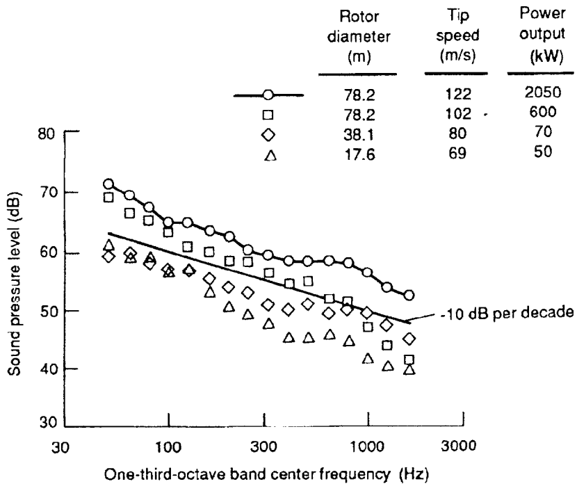
Figure 7-10. Noise spectra from small-, intermediate-, and large-scale HAWTs with downwind rotors (downwind distance = 2.5 rotor diameters) [Shepherd et al. 1988; Lungren 1984; Shepherd and Hubbard 1981; Hubbard and Shepherd 1982]
