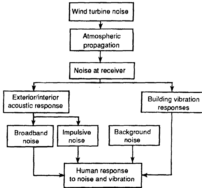
Figure 7-32. Method for evaluating human response to wind turbine noise [Stephens et al. 1982]
