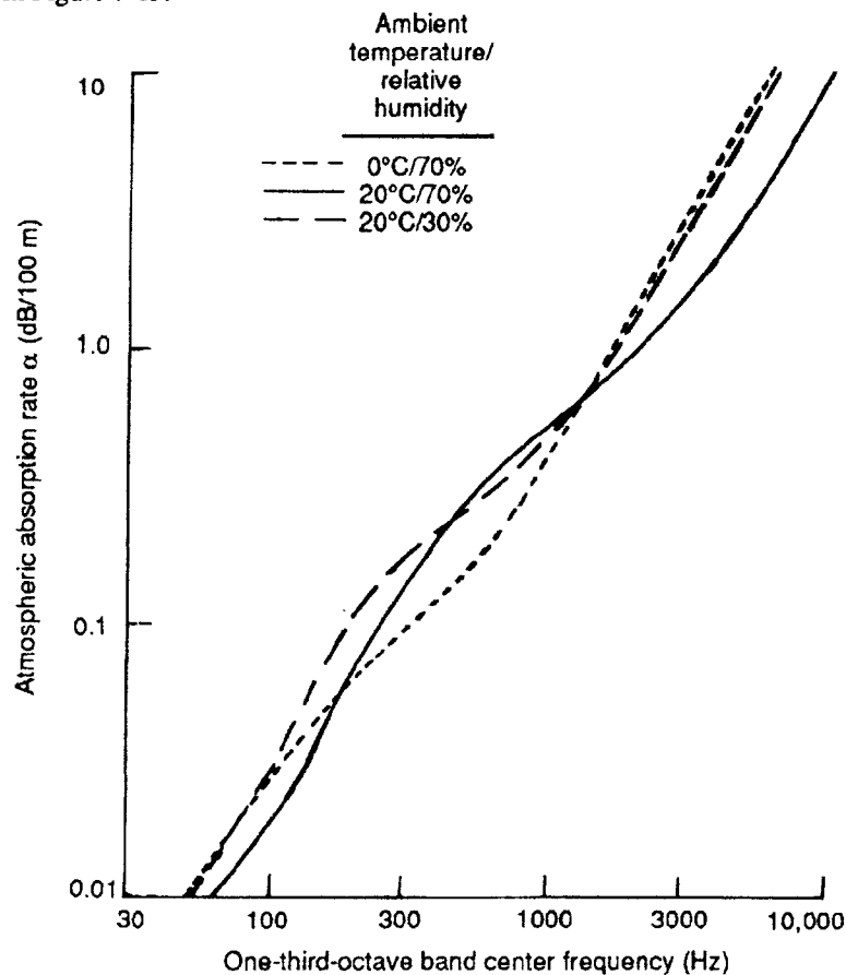
Figure 7-19. Standard rates of atmospheric absorption [ANSI 1978]
