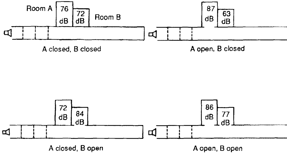
Figure 7-38. Effect of door positions on the maximum sound pressure levels in rooms adjacent to a hallway excited by a loudspeaker (21 Hz) [Hubbard and Shepherd 1986]
