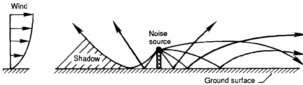
Figure 7-20. Effects of wind-induced refraction on acoustic rays radiating from an elevated point source [Shepherd and Hubbard 1985]
