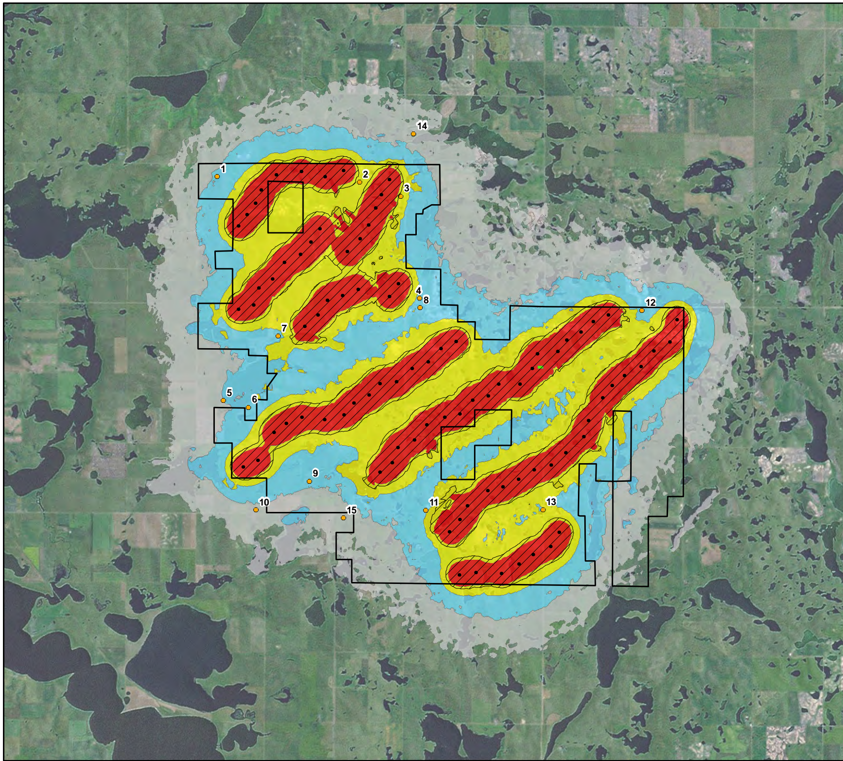
Figure 3a GE 2.5xl Received Sound Levels: Wind Turbines Operating at Maximum Rotation
