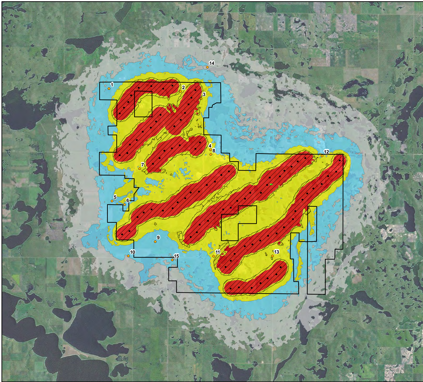
Figure 4b Siemens SWT-2.3-101 Received Sound Levels: Anomalous Meteorological Conditions Ashley Wind Energy Project McIntosh County, North Dakota
