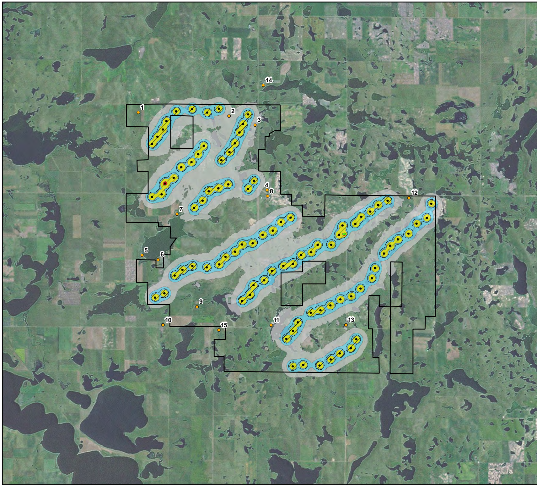
Figure 2b Siemens SWT-2.3-101 Received Sound Levels: Wind Turbines Operating at Cut-In Rotation
