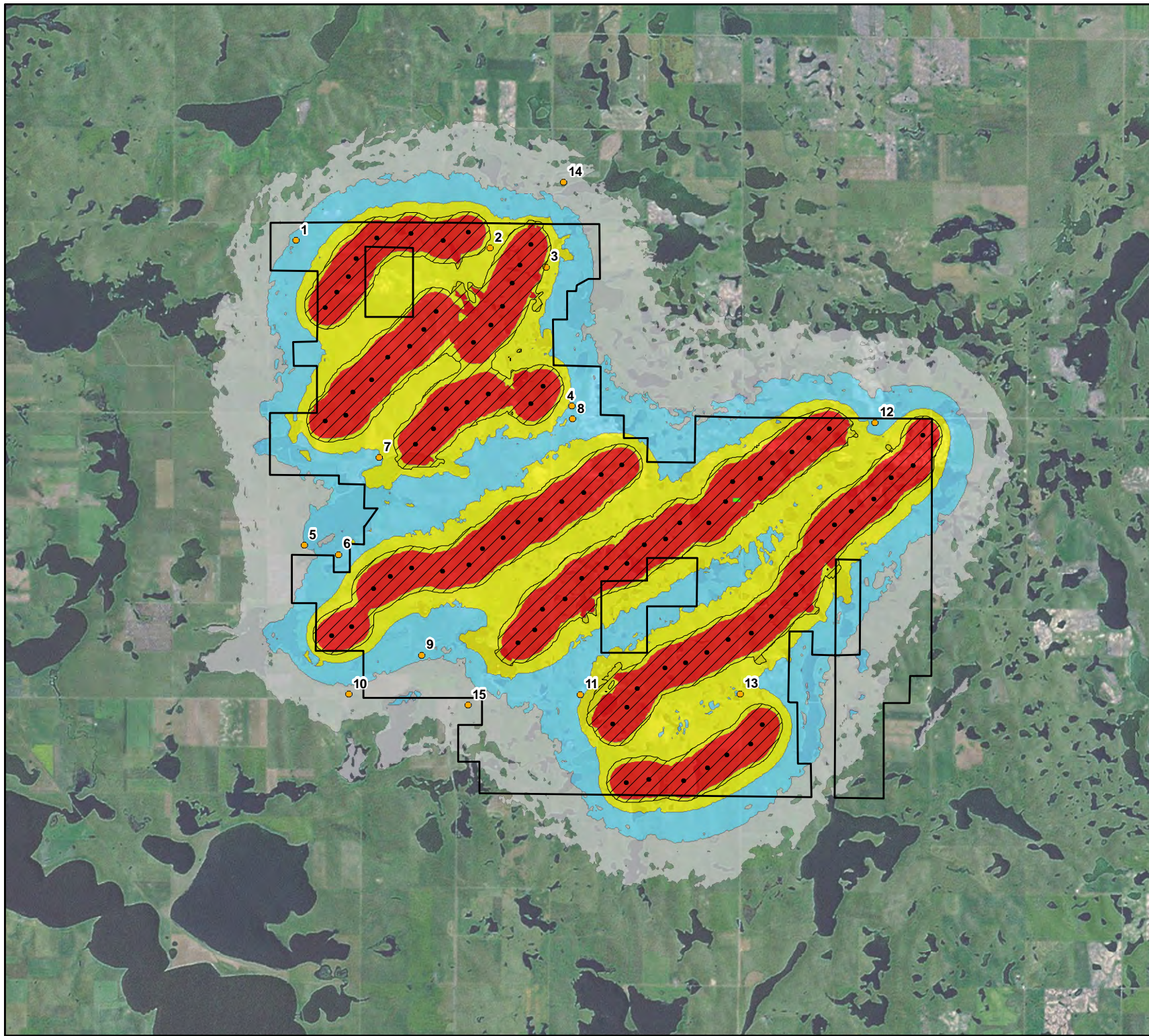
Figure 3b Siemens SWT-2.3-101 Received Sound Levels: Wind Turbines Operating at Maximum Rotation
