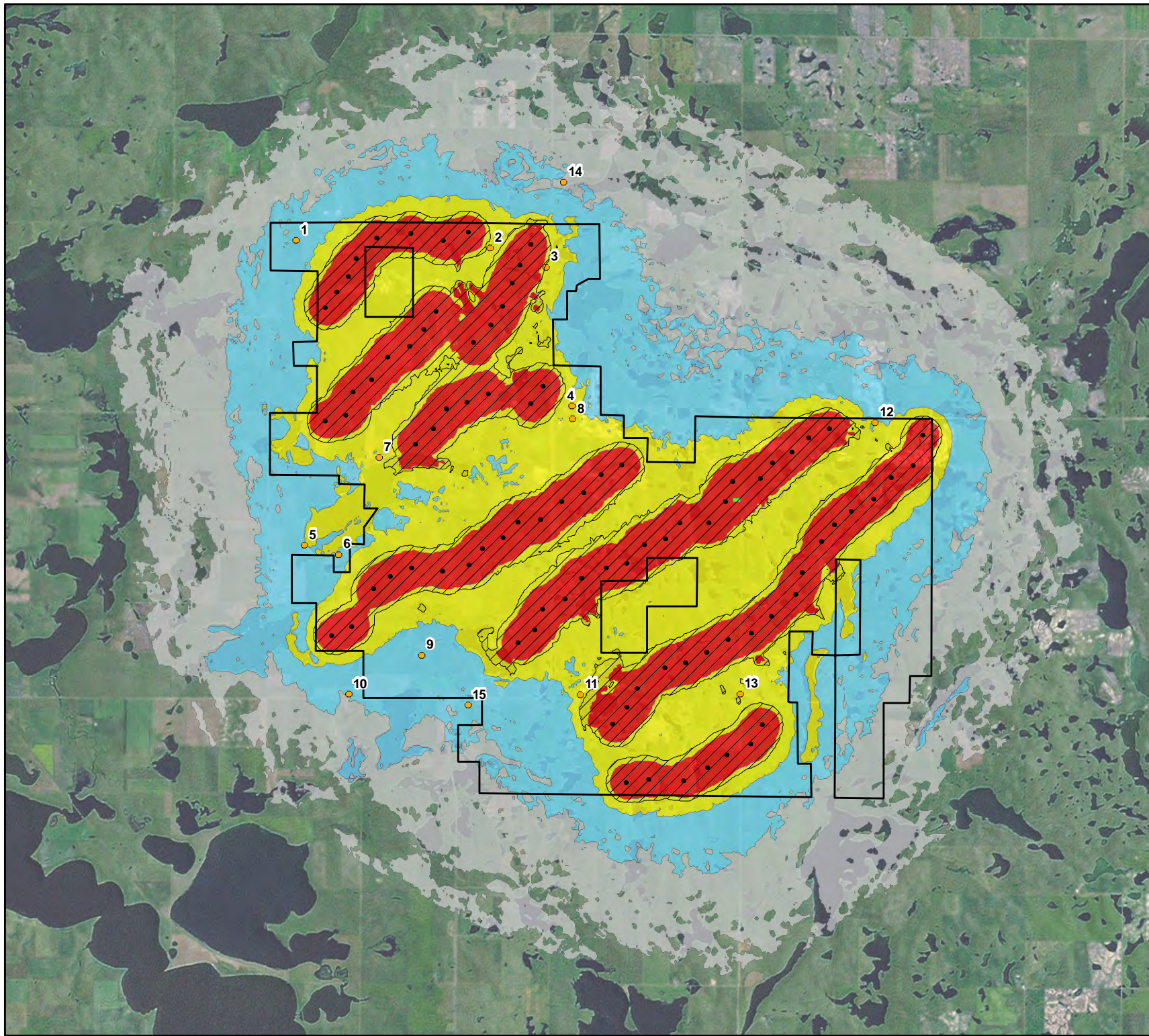
Figure 4a GE 2.5xl Received Sound Levels: Anomalous Meteorological Conditions
