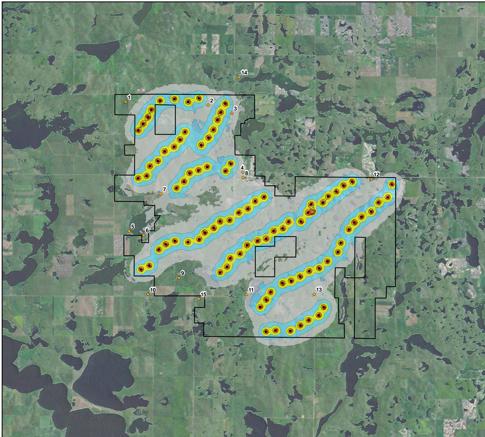
Figure 2a GE 2.5xl Received Sound Levels: Wind Turbines Operating at Cut-In Rotation
