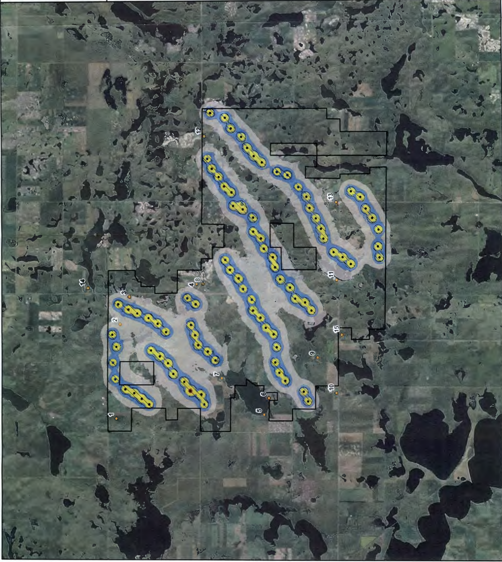
Figure 2b Siemens SWT-2.3-101 Received Sound Levels: Wind Turbines Operating at Cut-in Rotation
