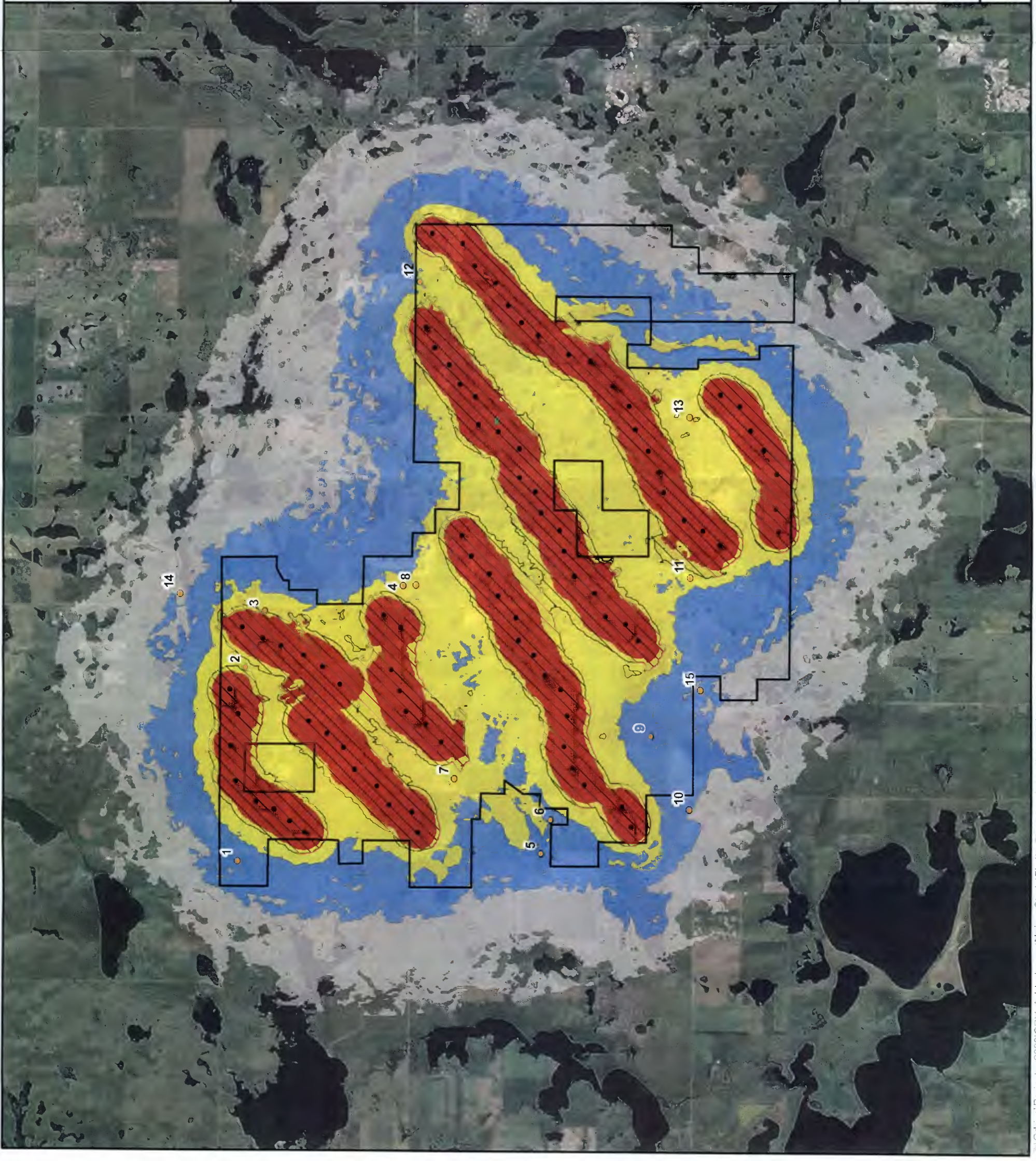
Figure 4b Siemens SWT-2.3-101 Received Sound Levels: Anomalous Meteorological Conditions
