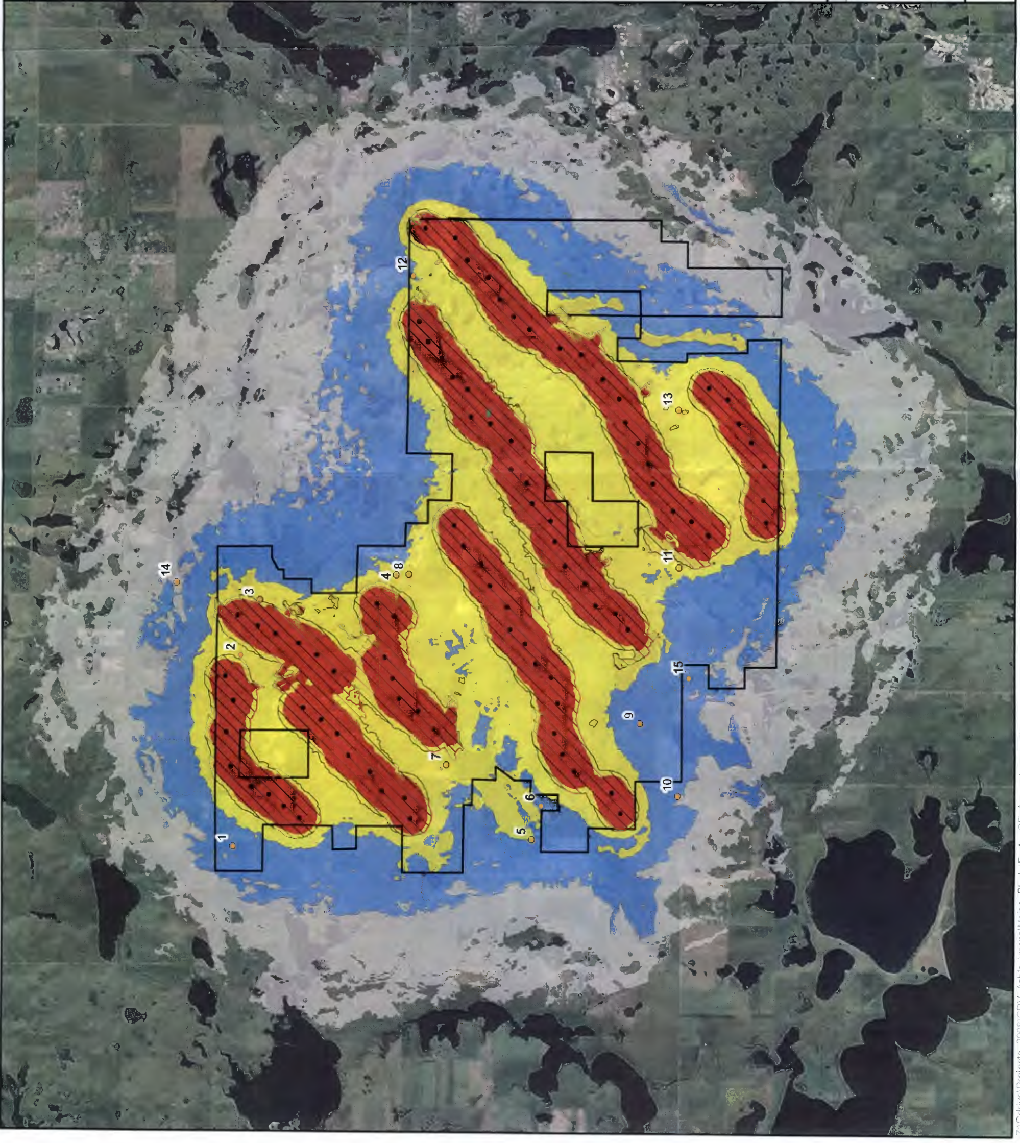
Figure 4a GE 2.5xl Received Sound Levels: Anomalous Meteorological Conditions
