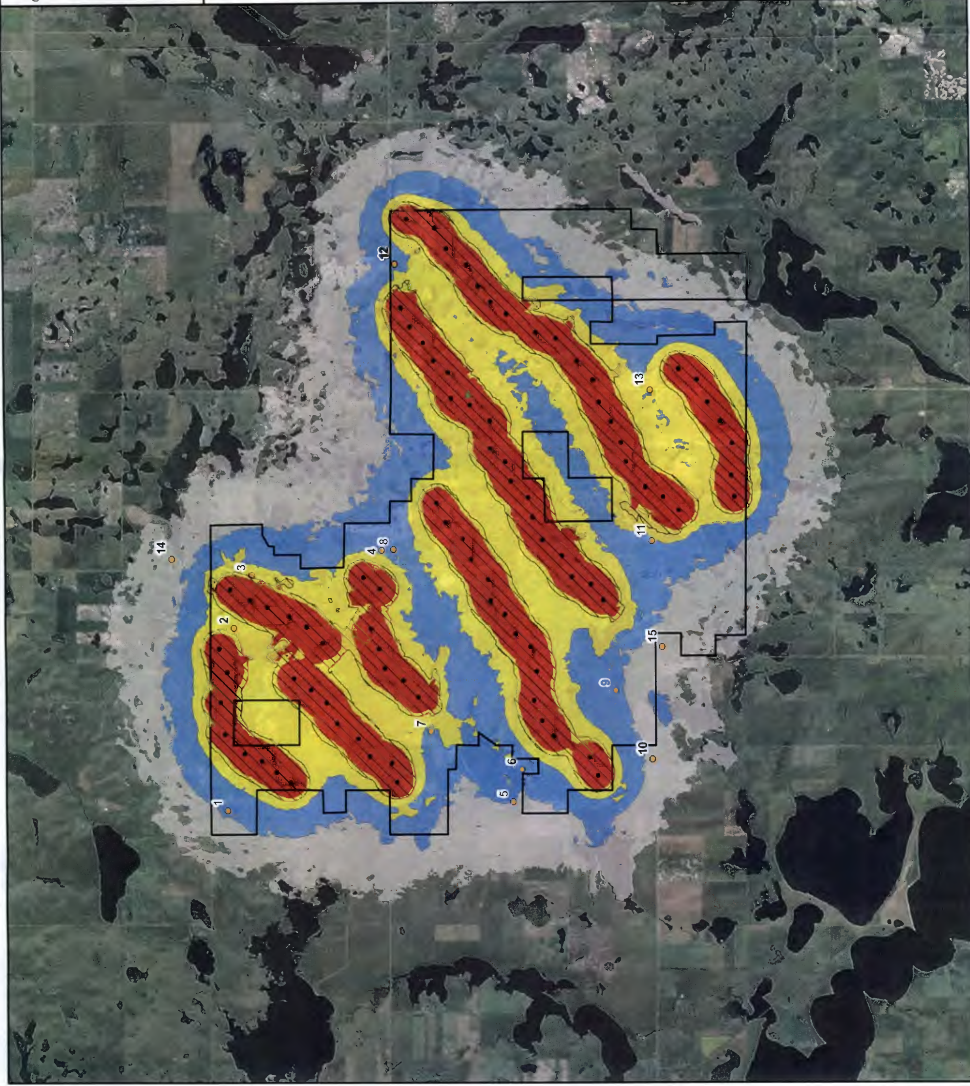
Figure 3a GE 2.5xl Received Sound Levels: Wind Turbines Operating at Maximum Rotation
