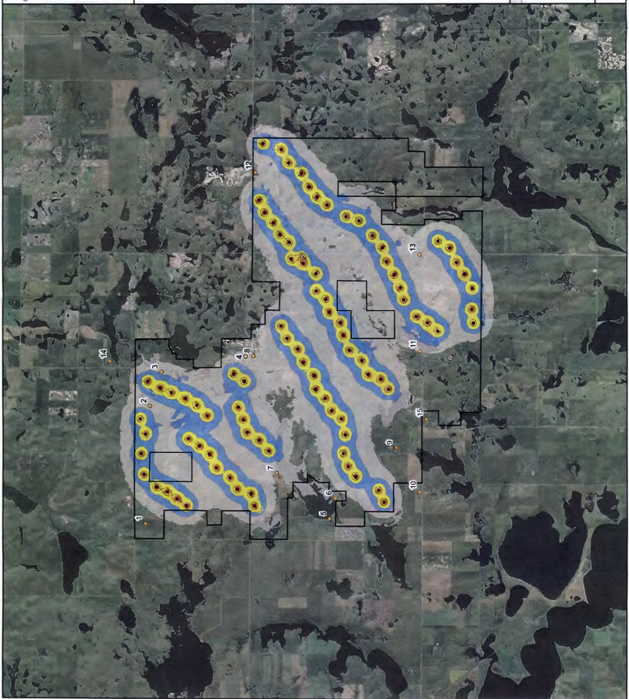
Figure 2a GE 2.5xl Received Sound Levels: Wind Turbines Operating at Cut-In Rotation
