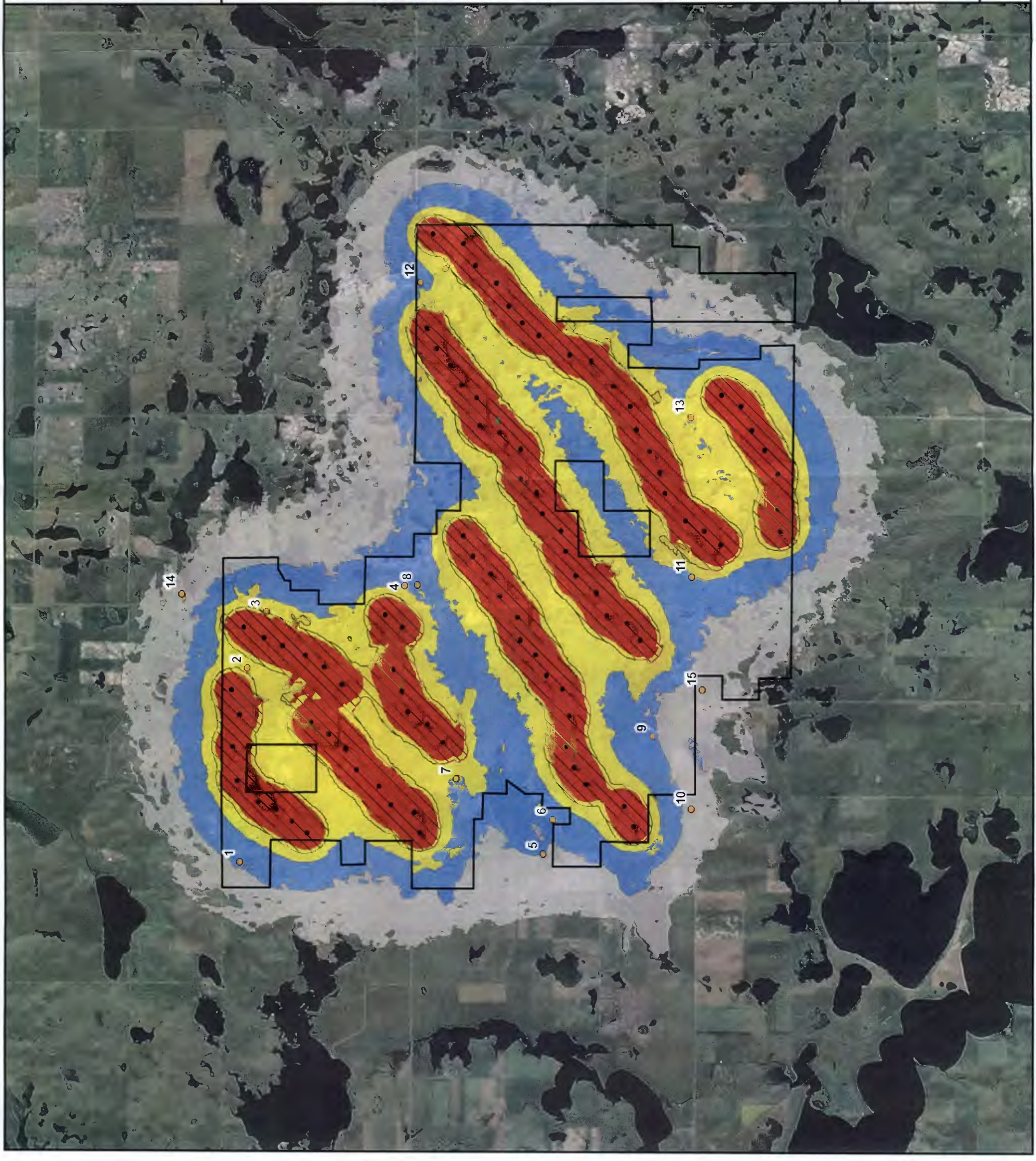
Figure 3b Siemens SWT-2.3-101 Received Sound Levels: Wind Turbines Operating at Maximum Rotation
