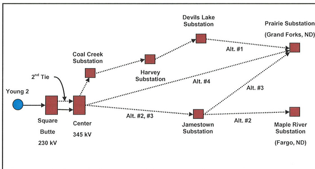
Figure 3-3. New 345 kV Center to Red River Valley Line Alternatives for Preliminary Near-Term Analysis
