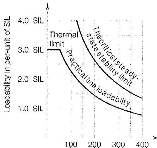
Figure 3-1. Transmission Line Loadability Limits
