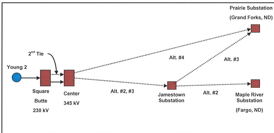
Figure 3-4. New 345 kV Center to Red River Valley Line Alternatives for Voltage Stability Analysis
