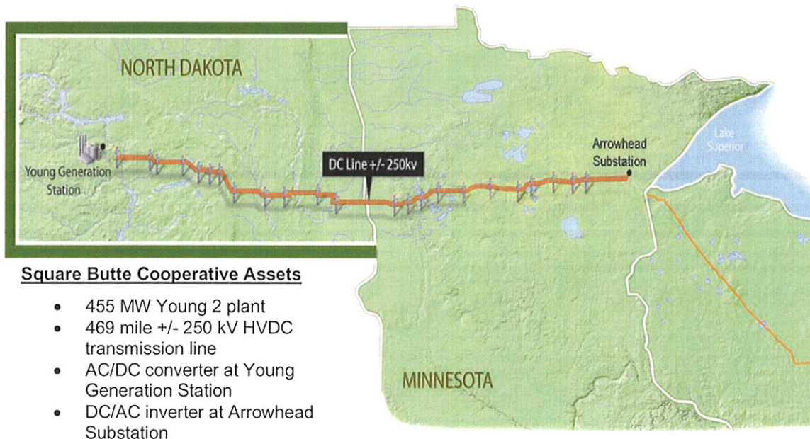
Figure 1-2. Square Butte Cooperative Assets
