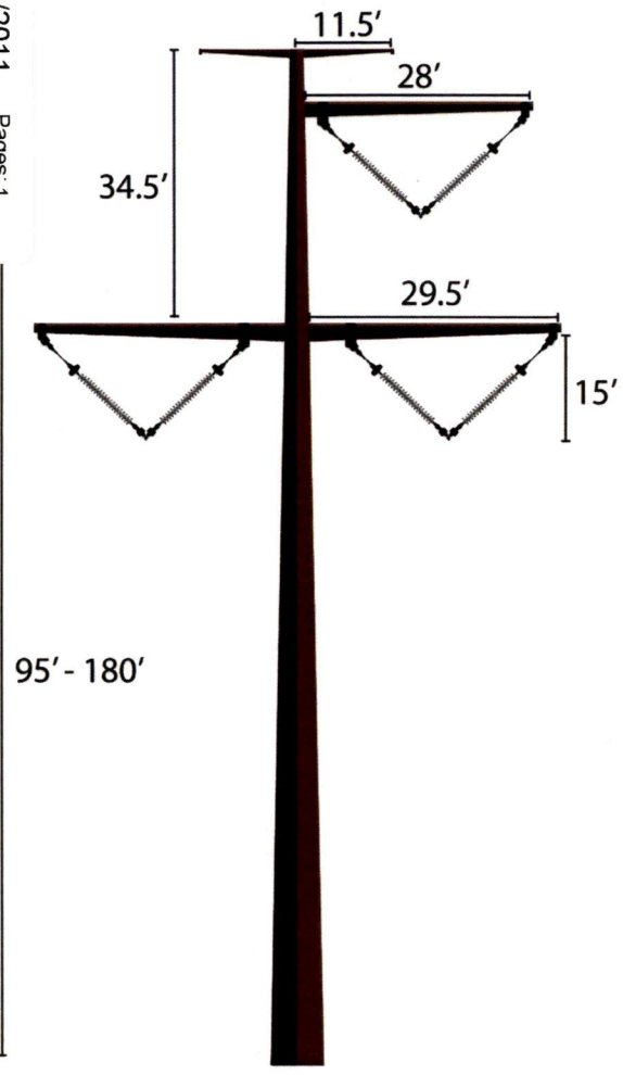
Typical Monopole
