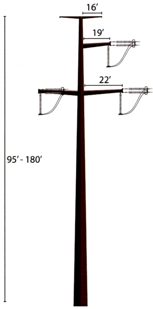
Dead-End Monopole
