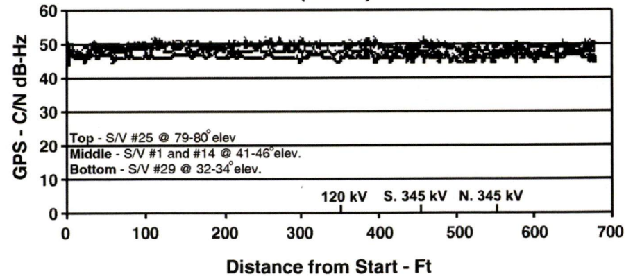
GPS C/N vs Distance Across 120/345/345 kV Easement (Site #2)
