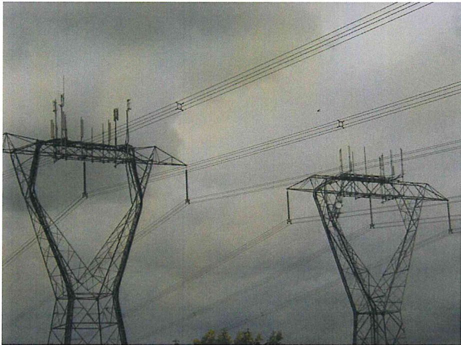
Communications Antennas mounted on 500 kV transmission lines
