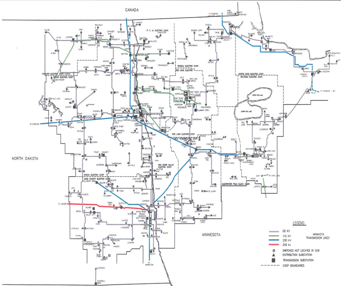
Figure 2-2. Minnkota Transmission System
