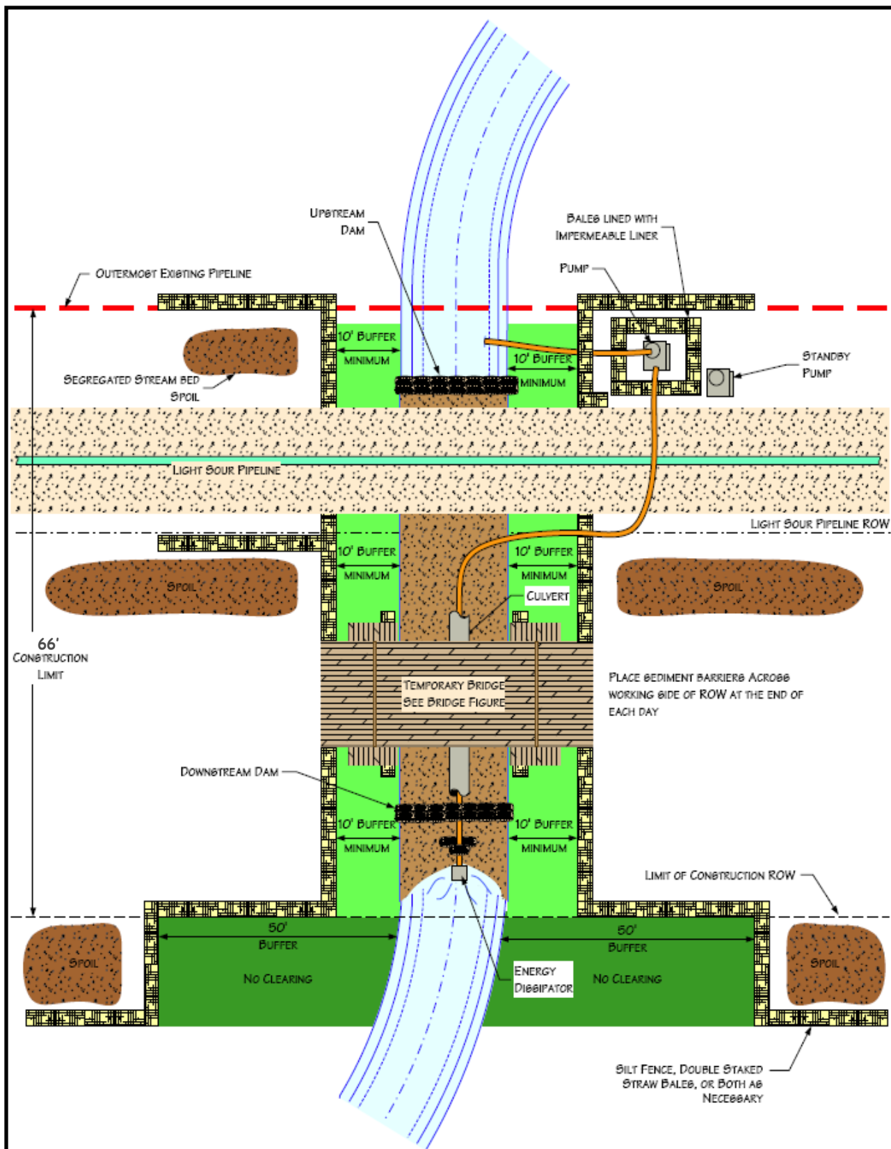
Figure 6.2.2 – Typical Waterbody Crossing Dam and Pump Method 12-inch Crude Oil Pipeline July 2010
