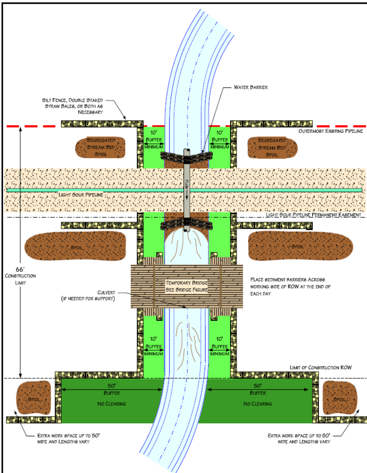
Figure 6.2.3 – Typical Waterbody Crossing Flume Method 12-inch Crude Oil Pipeline July 2010
