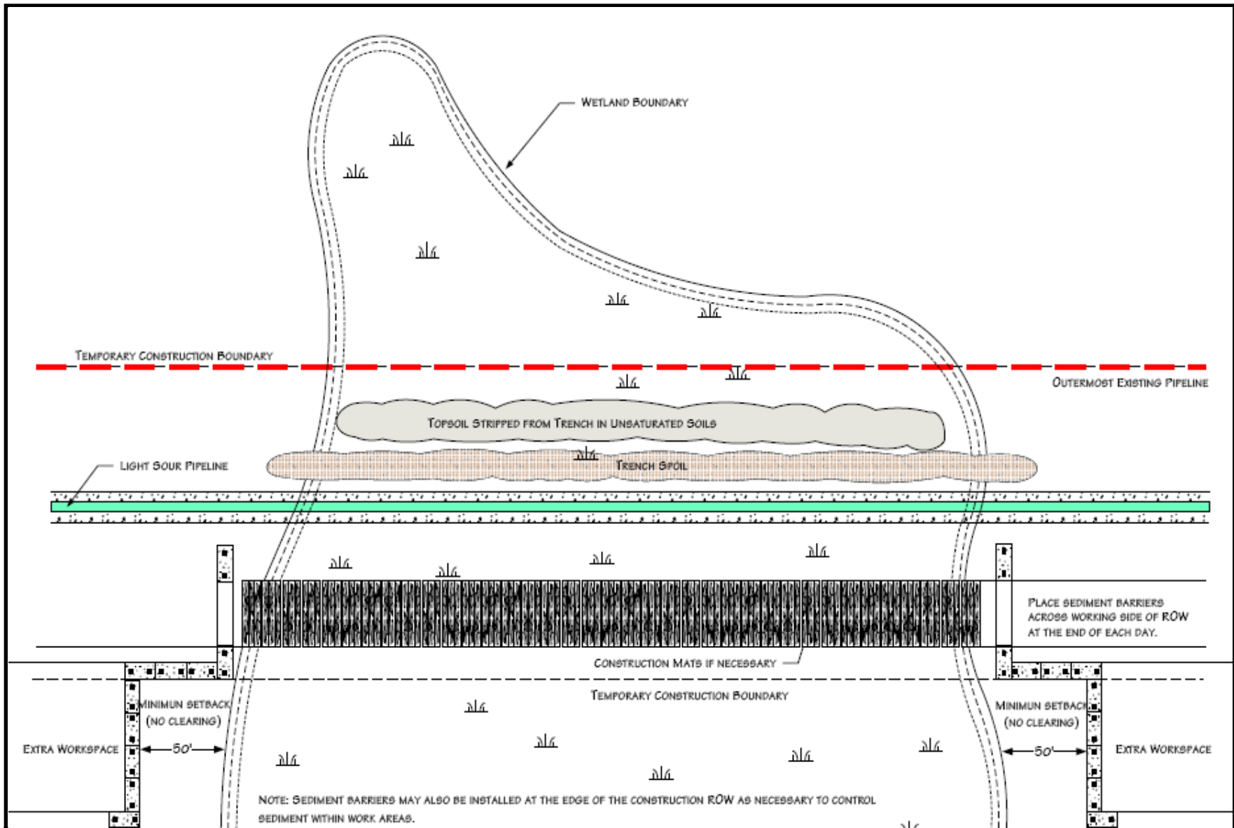
Figure 6.3.1 – Typical Wetland Crossing Method 12-inch Crude Oil Pipeline July 2010
