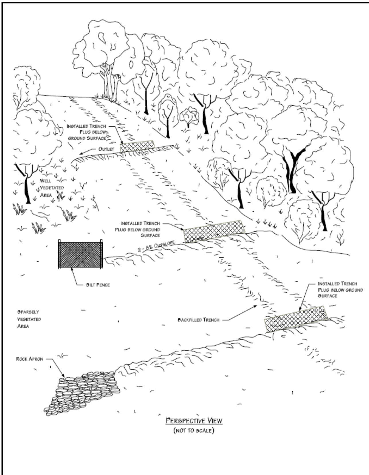
Figure 6.7.1 – Permanent Slope Breakers Perspective View 12-inch Crude Oil Pipeline July 2010
