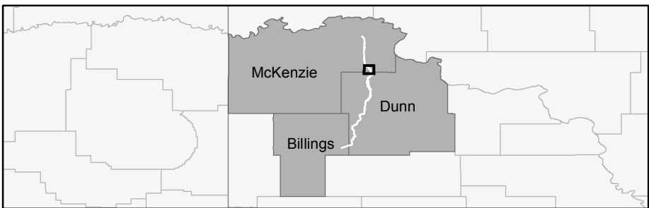
Figure 4.B.5a - Route Map 12-Inch Crude Oil Pipeline Township 149 Range 95 July 2010
