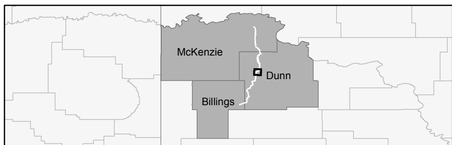
Figure 4.B.9a - Route Map 12-Inch Crude Oil Pipeline Township 146 Range 96 July 2010
