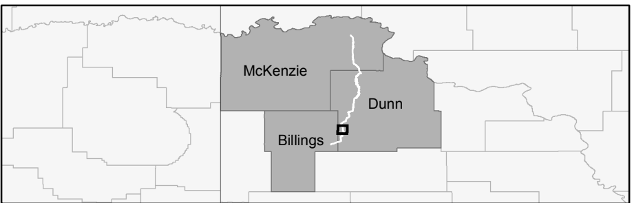
Figure 4.B.13a - Route Map 12-Inch Crude Oil Pipeline Township 143 Range 97 July 2010
