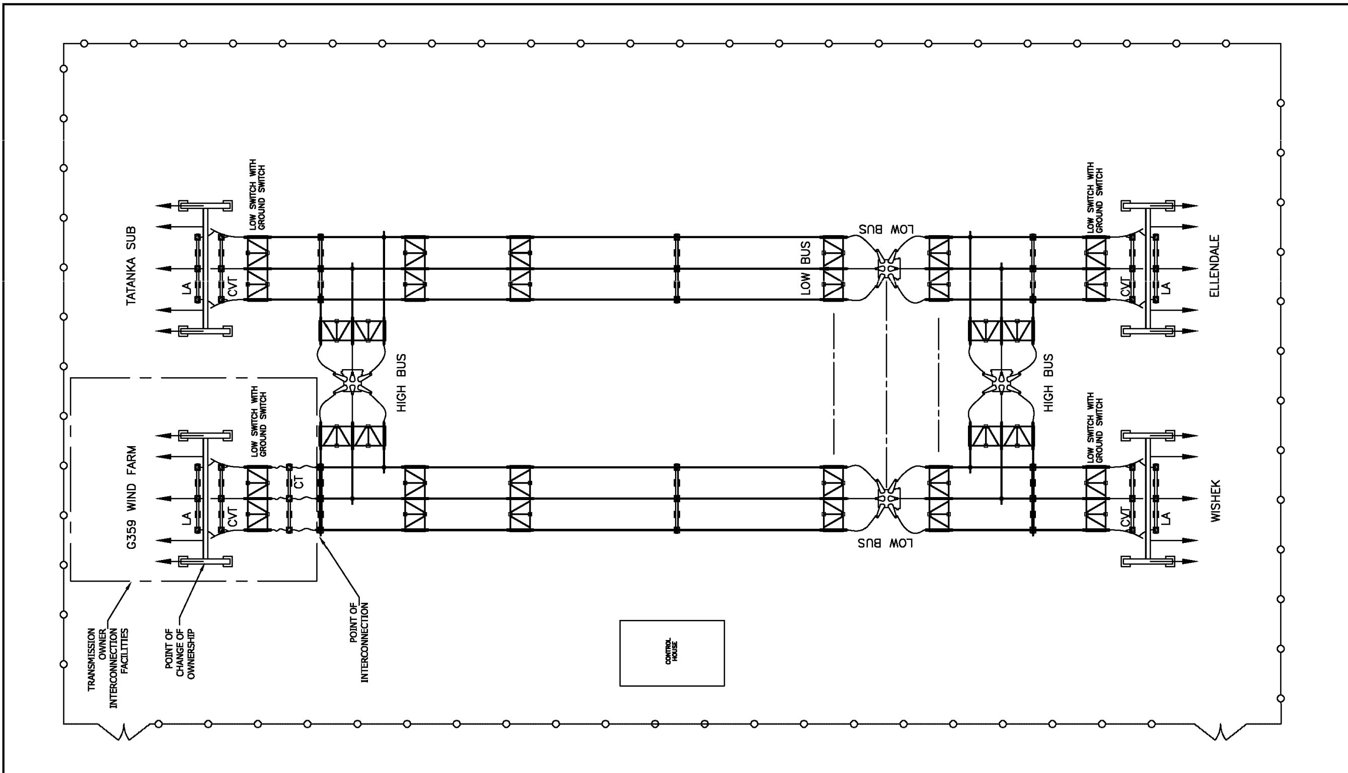
Exhibit A3-1 – G359 Interconnect General Arrangement
