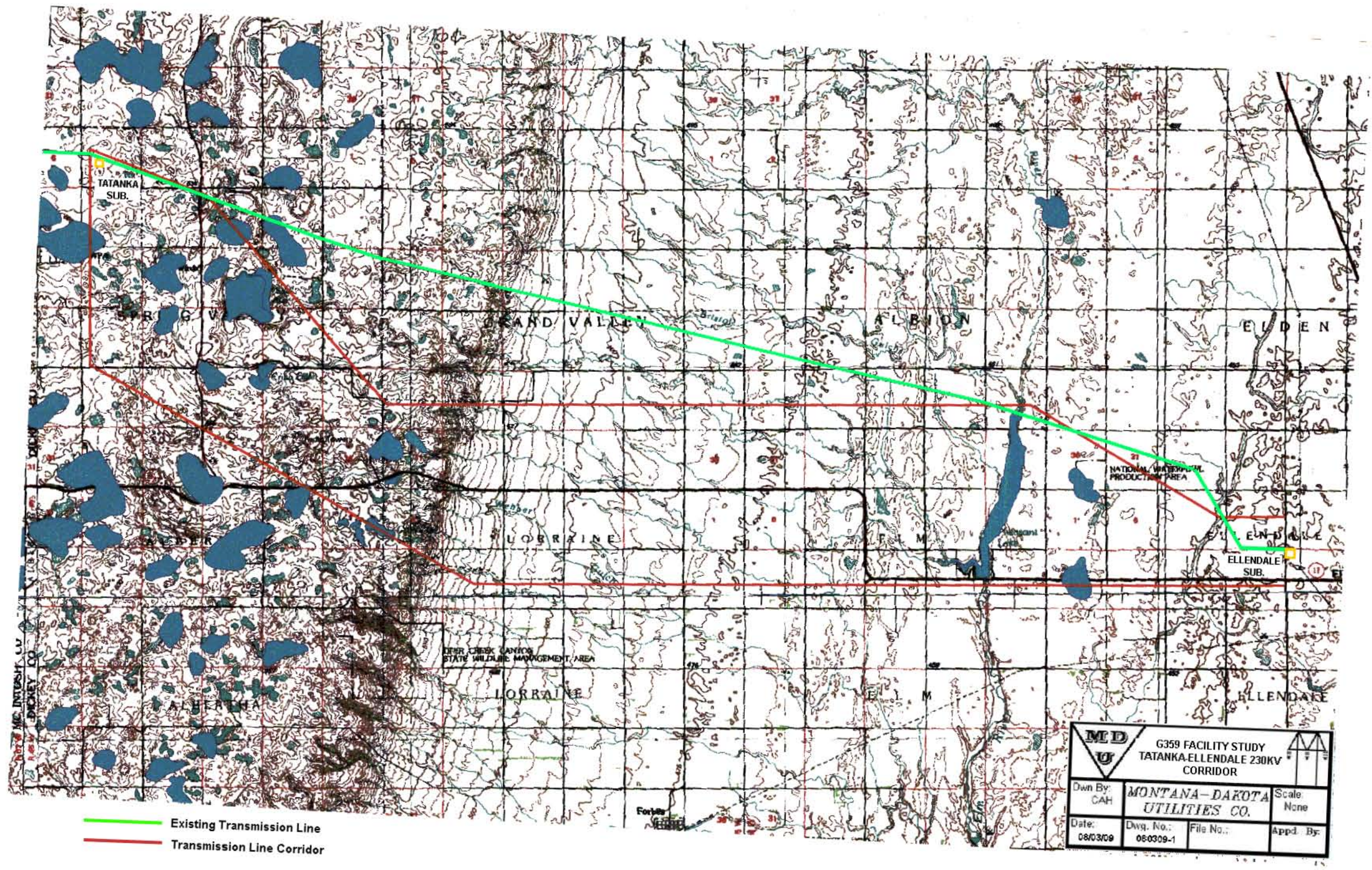
Exhibit A4 – Transmission Line Plan and Profile – Corridor Drawing
