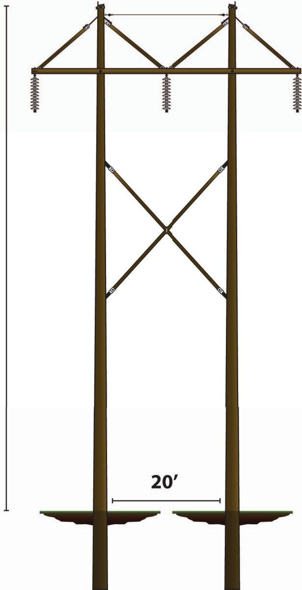
Single Circuit H-Frame
