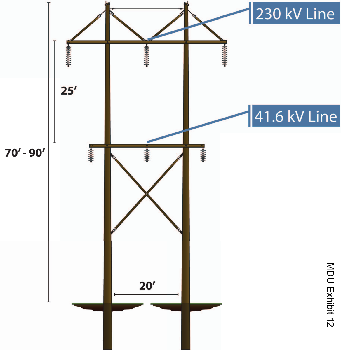
Double Circuit H-Frame
