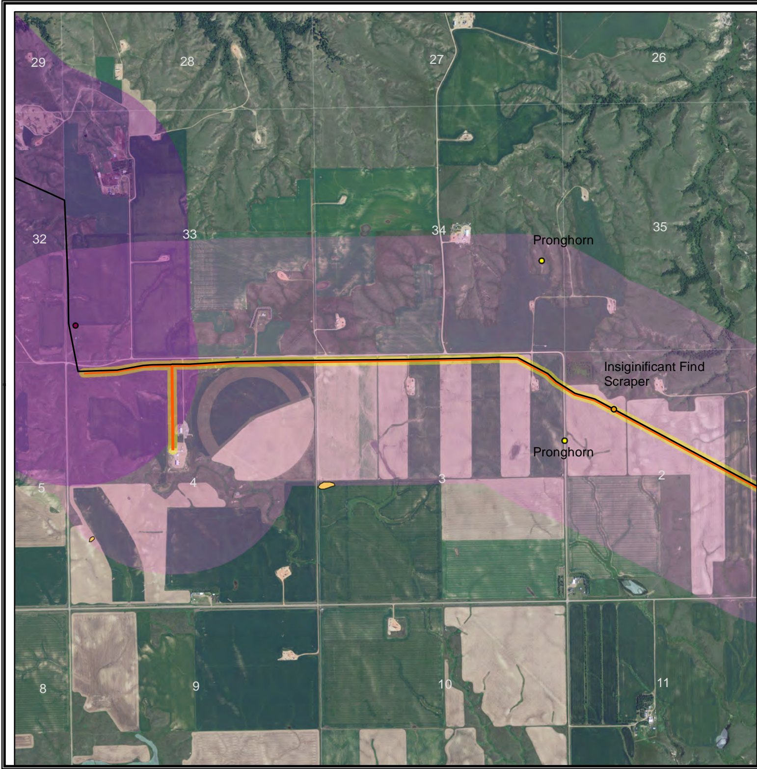
Figure 4.A.2a - Route Map 6-Inch Natural Gas Liquids Pipeline McKenzie County Township 152 Range 103 Township 151 Range 103 July 2011
