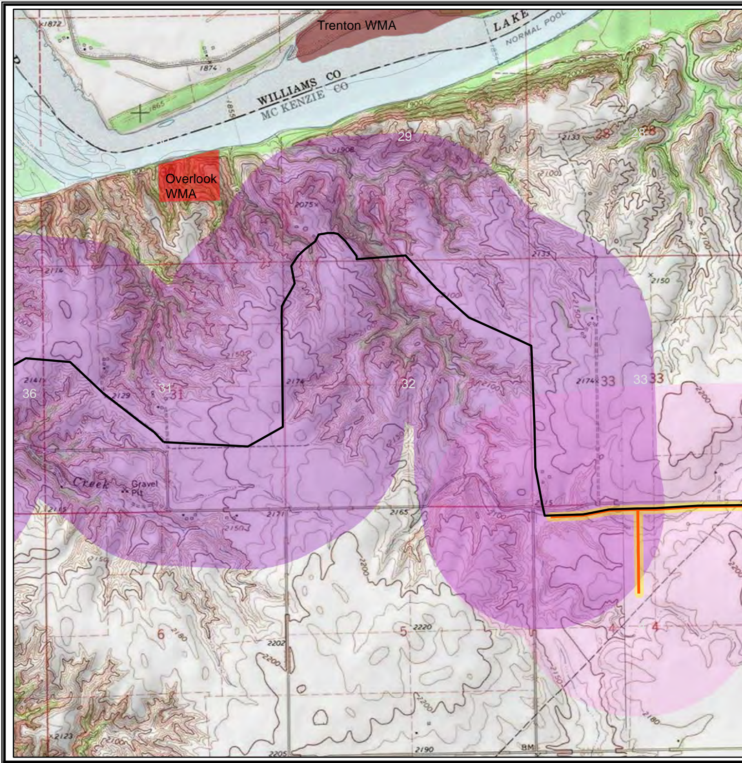
Figure 4.A.3b - Route Map 6-Inch Natural Gas Liquids Pipeline McKenzie County Township 151N Range 103W Township 152N Range 103W July 2011
