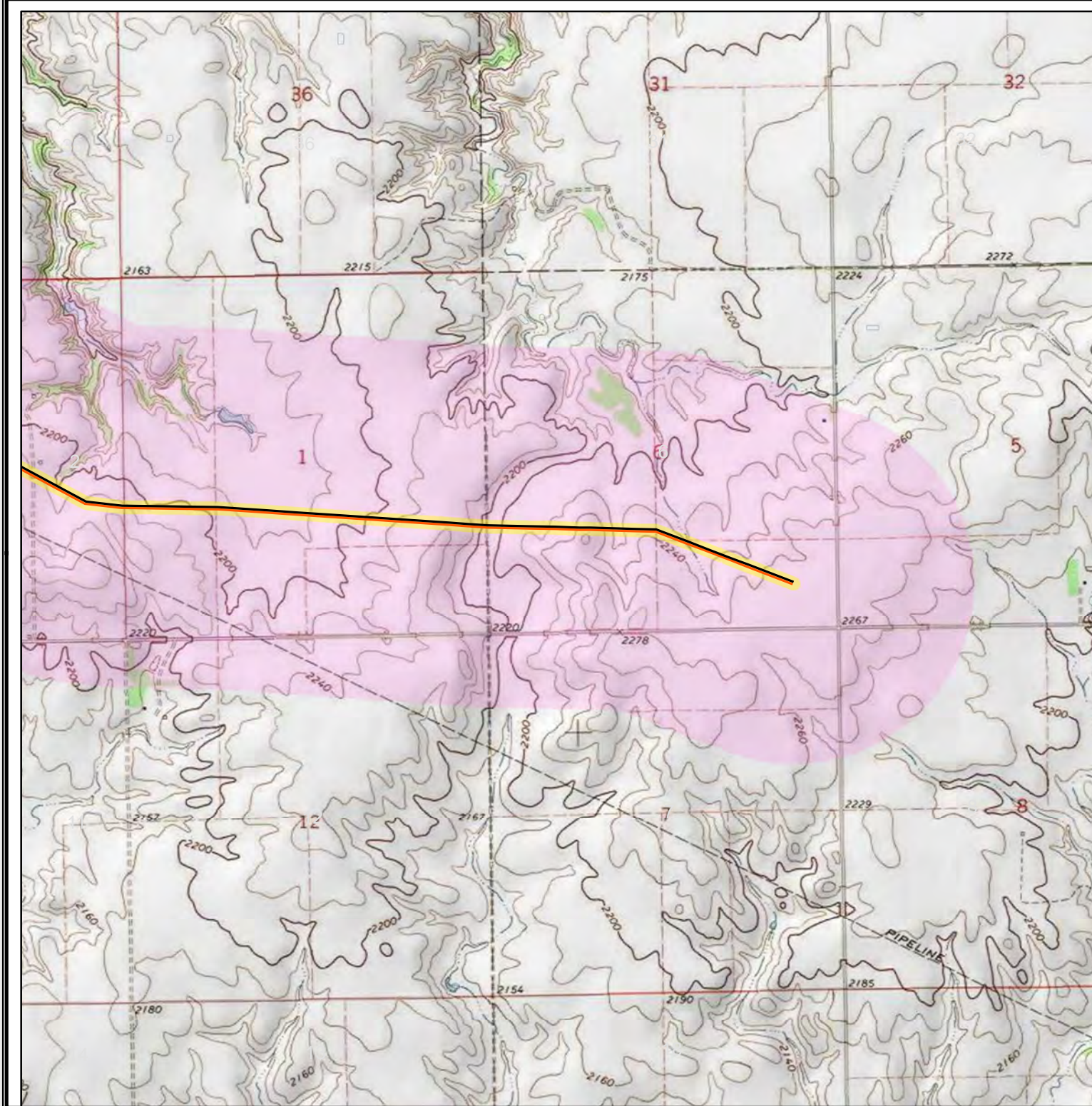
Figure 4.A.1b - Route Map 6-Inch Natural Gas Liquids Pipeline McKenzie County Township 152 Range 103 Township 152 Range 102 Township 151 Range 103 Township 151 Range 102 July 2011
