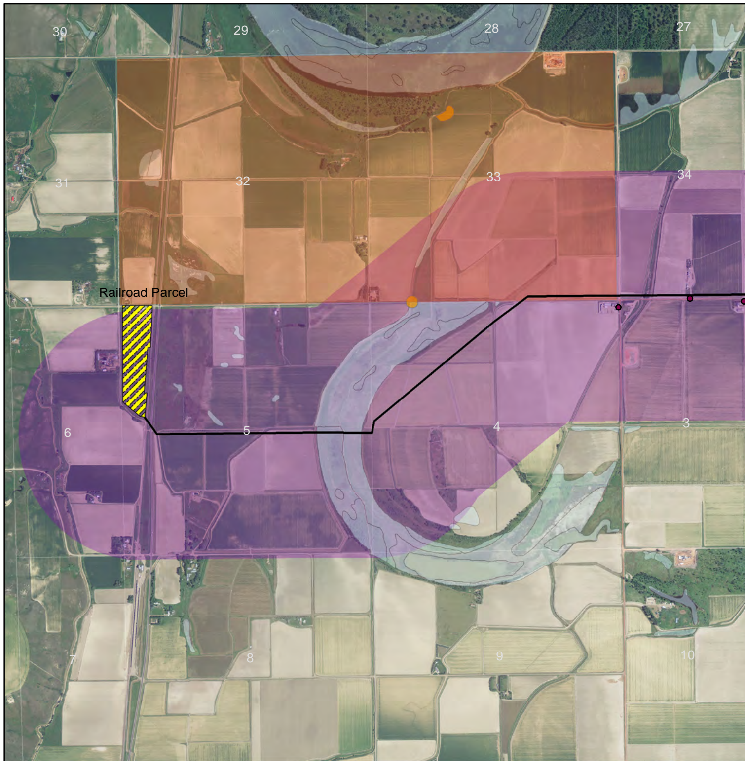
Figure 4.A.5a - Route Map 6-Inch Natural Gas Liquids Pipeline McKenzie County Township 151N Range 104W Township 152N Range 104W July 2011
