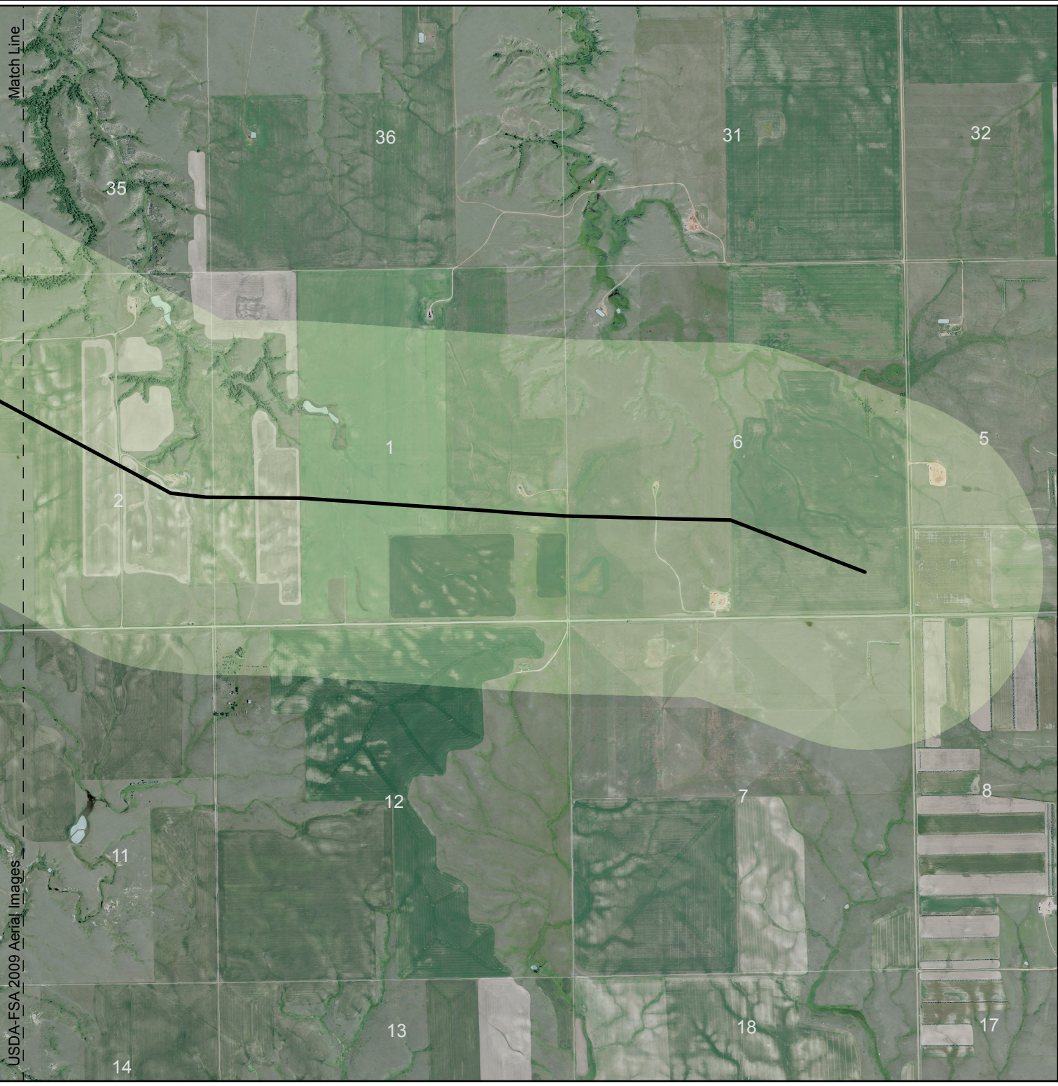
Figure 4.A.1a - Route Map 8-Inch Natural Gas Pipeline Township 151N Range 102W October 2010
