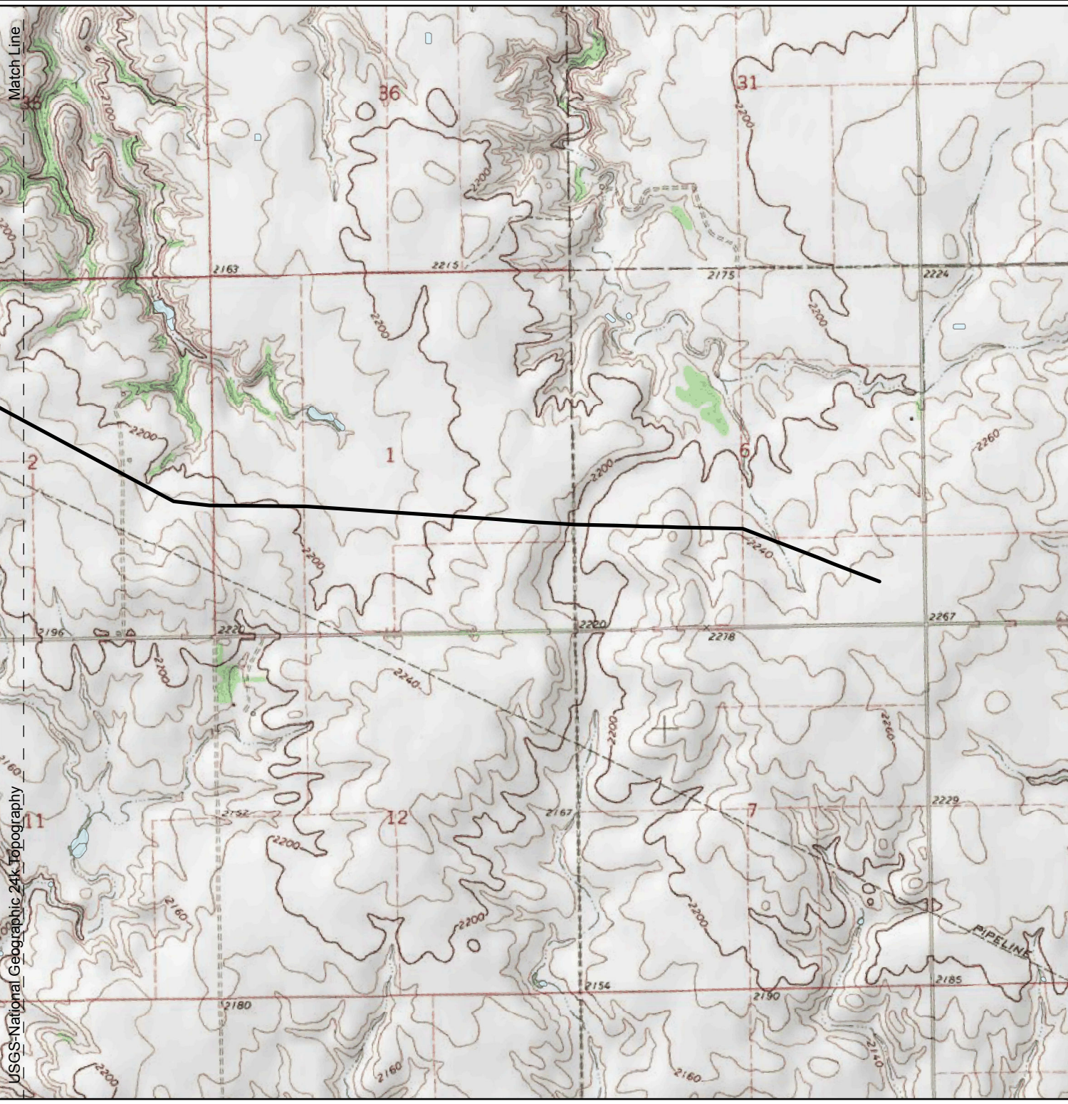
Figure 4.A.1b - Route Map 8-Inch Natural Gas Pipeline Township 151N Range 102W October 2010
