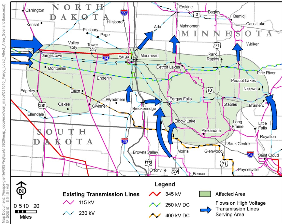
Figure 5 South Zone of the Red River Valley area and Flows on High Voltage Transmission Lines
