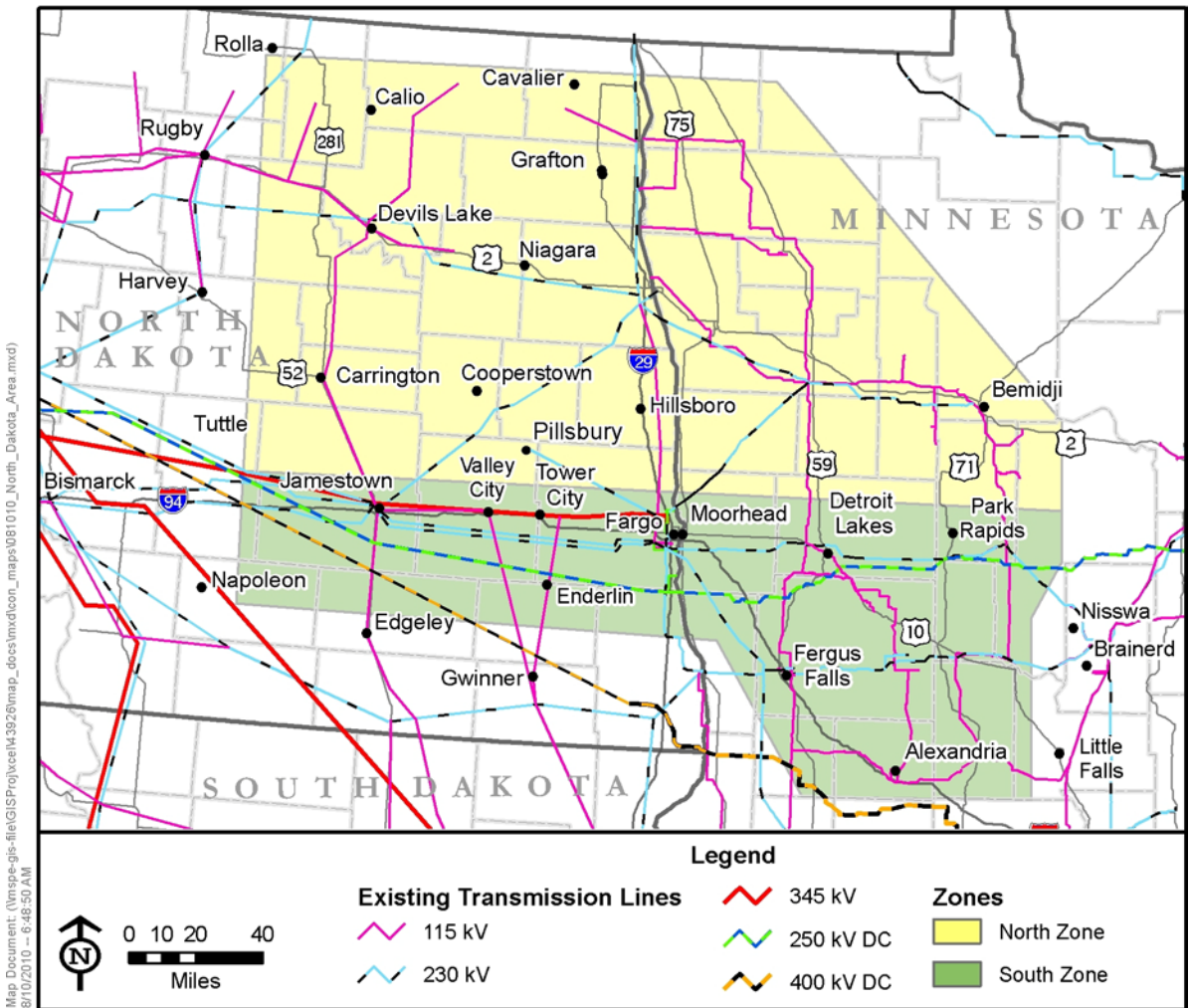
Figure 4 Red River Valley Area
