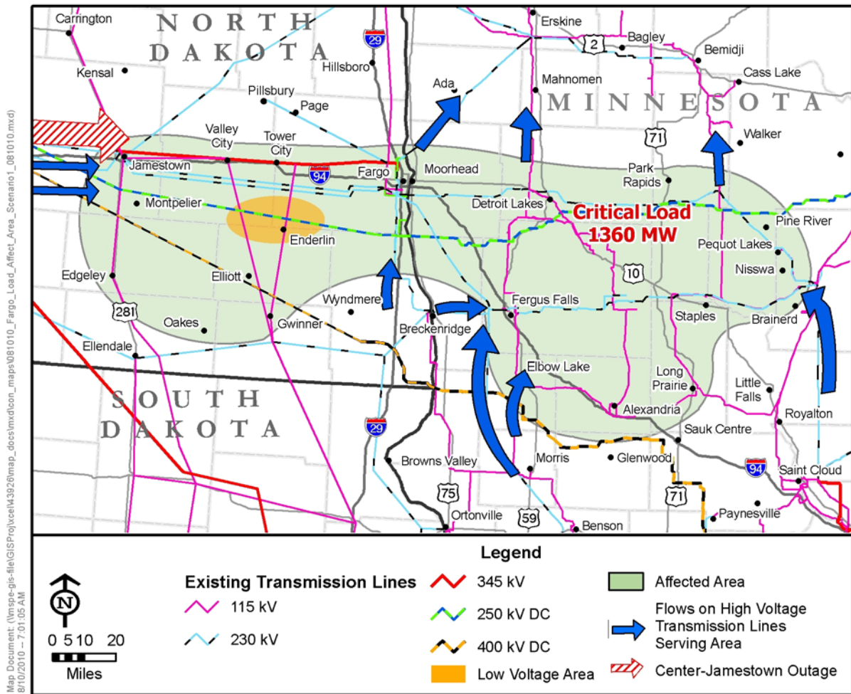
Figure 6 Center – Jamestown 345 kV Contingency
