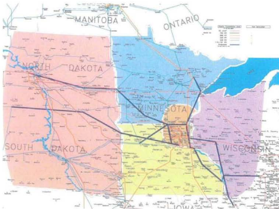
Diagram 15 – Eastern Bias Preliminary Recommended Facilities
