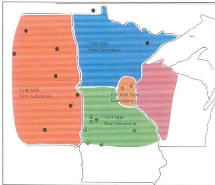
Diagram 6 - North/West Bias Generation Locations
