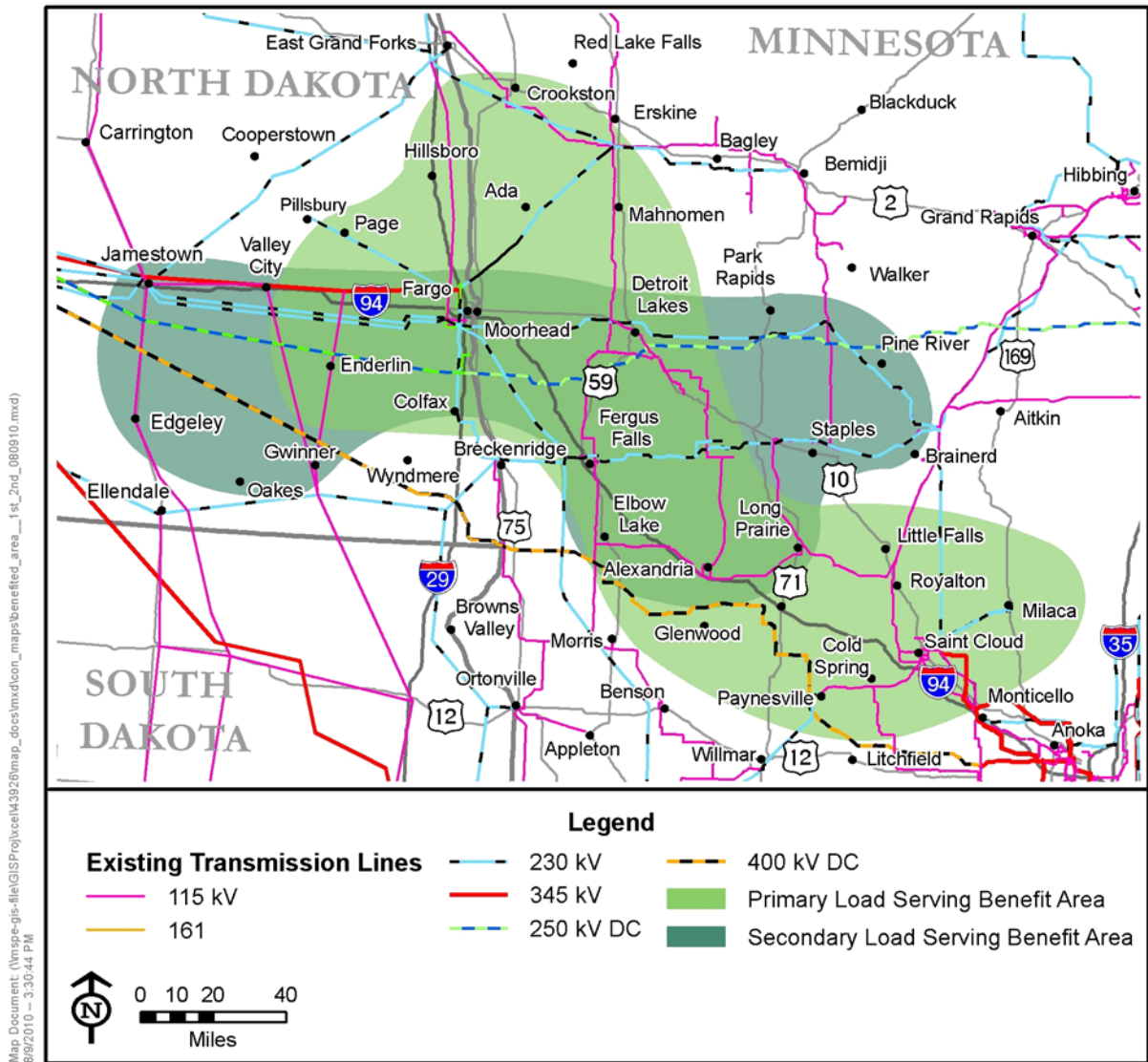
Figure 7 Fargo – Twin Cities 345 kV Load Serving Benefit Areas
