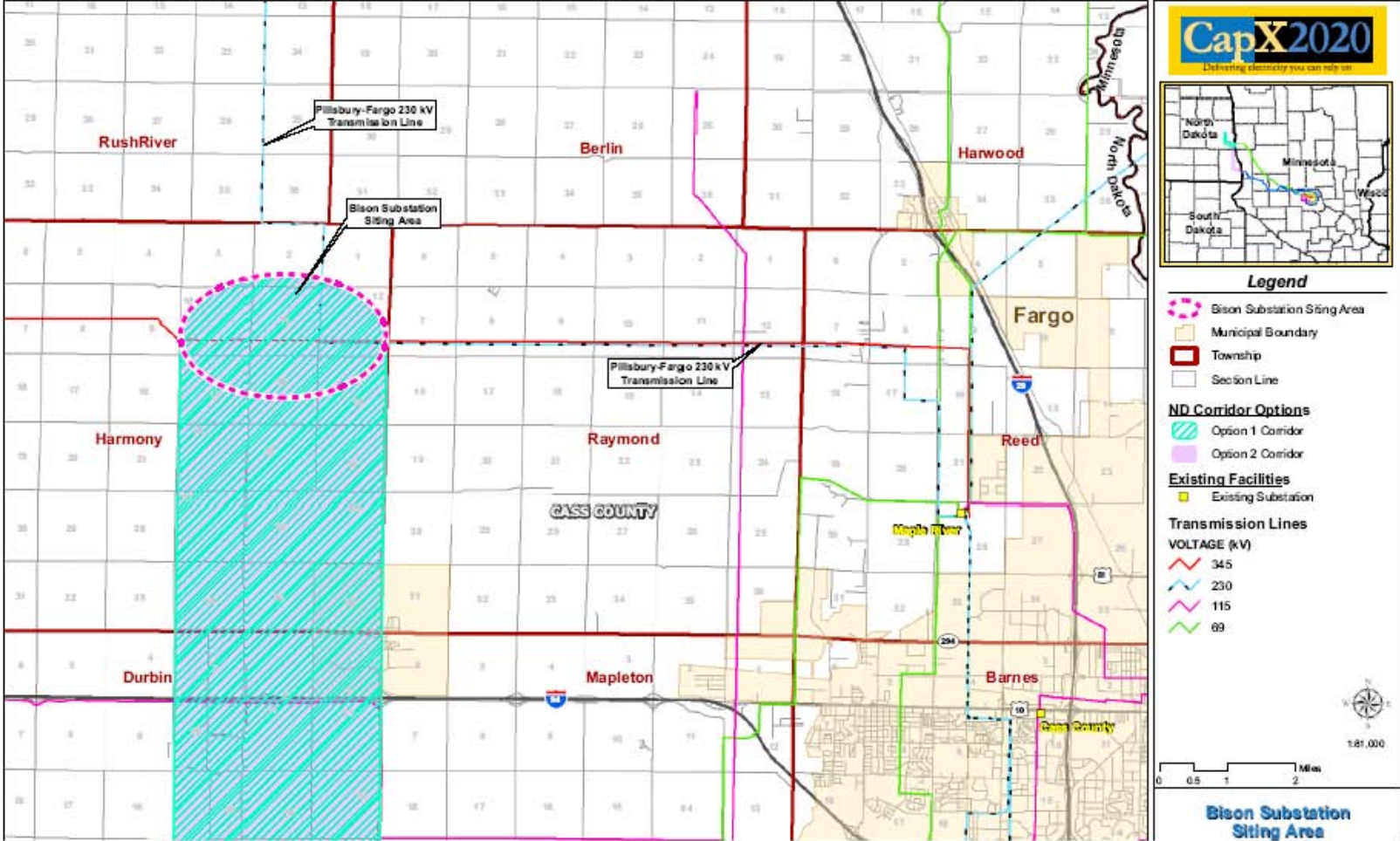
Figure 2 Bison Substation Location
