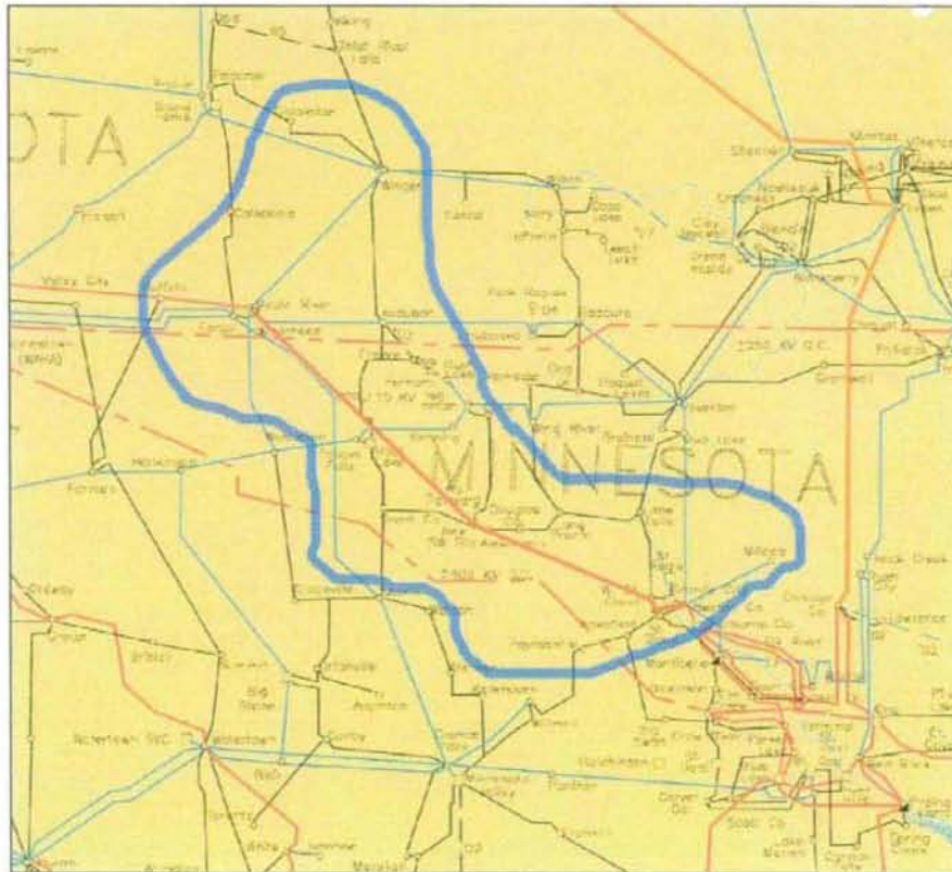
Diagram 5.4.A Load Benefit Area for the Fargo-St. Cloud 345 kV Line Addition
