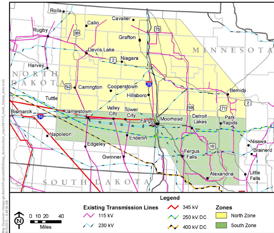
Figure 1 HVTLs in North Dakota
