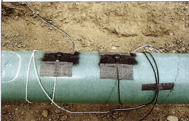
Test Leads
