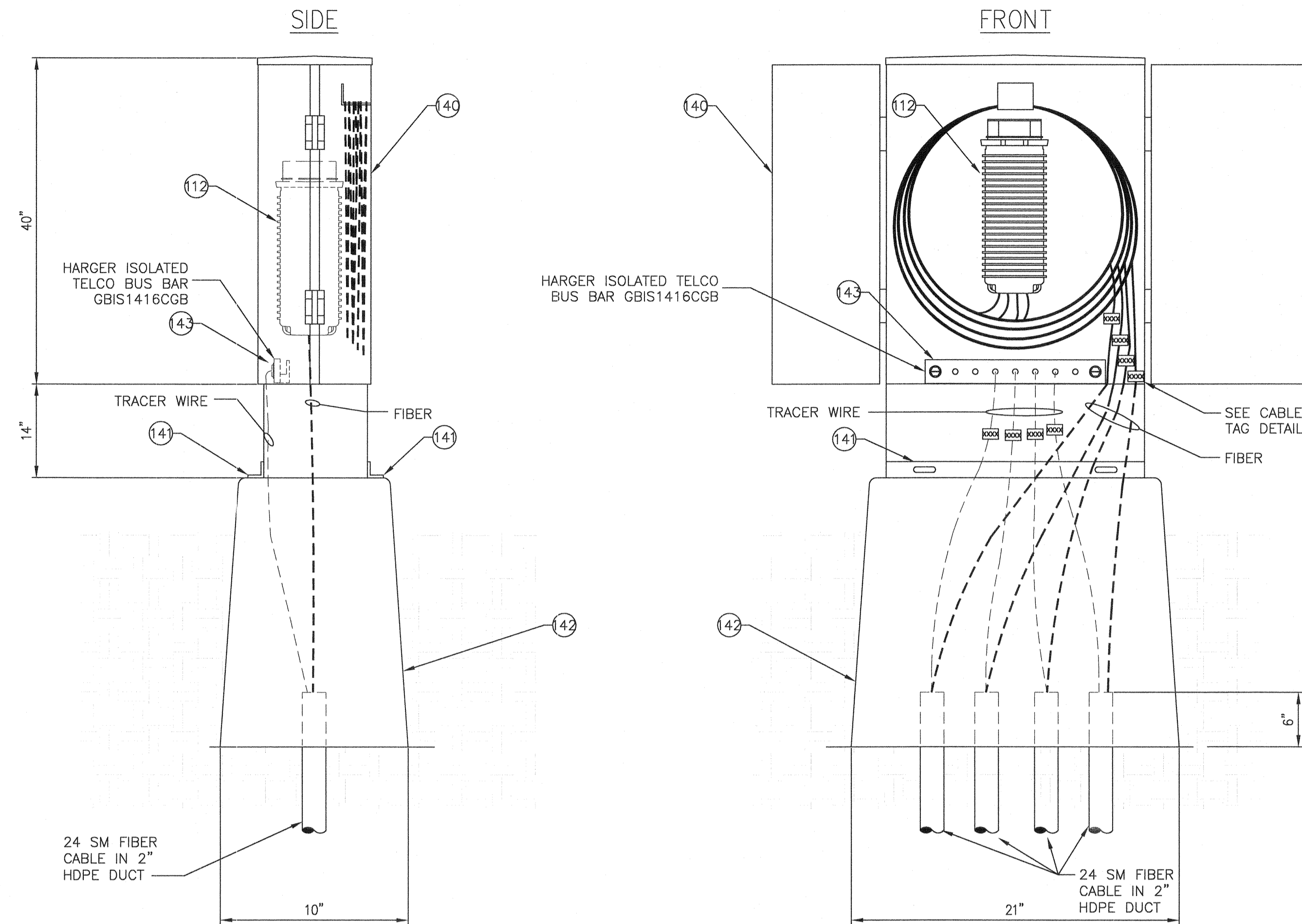
SPLICE ENCLOSURE DETAIL ABOVE GRADE 4-WAY N.T.S.
