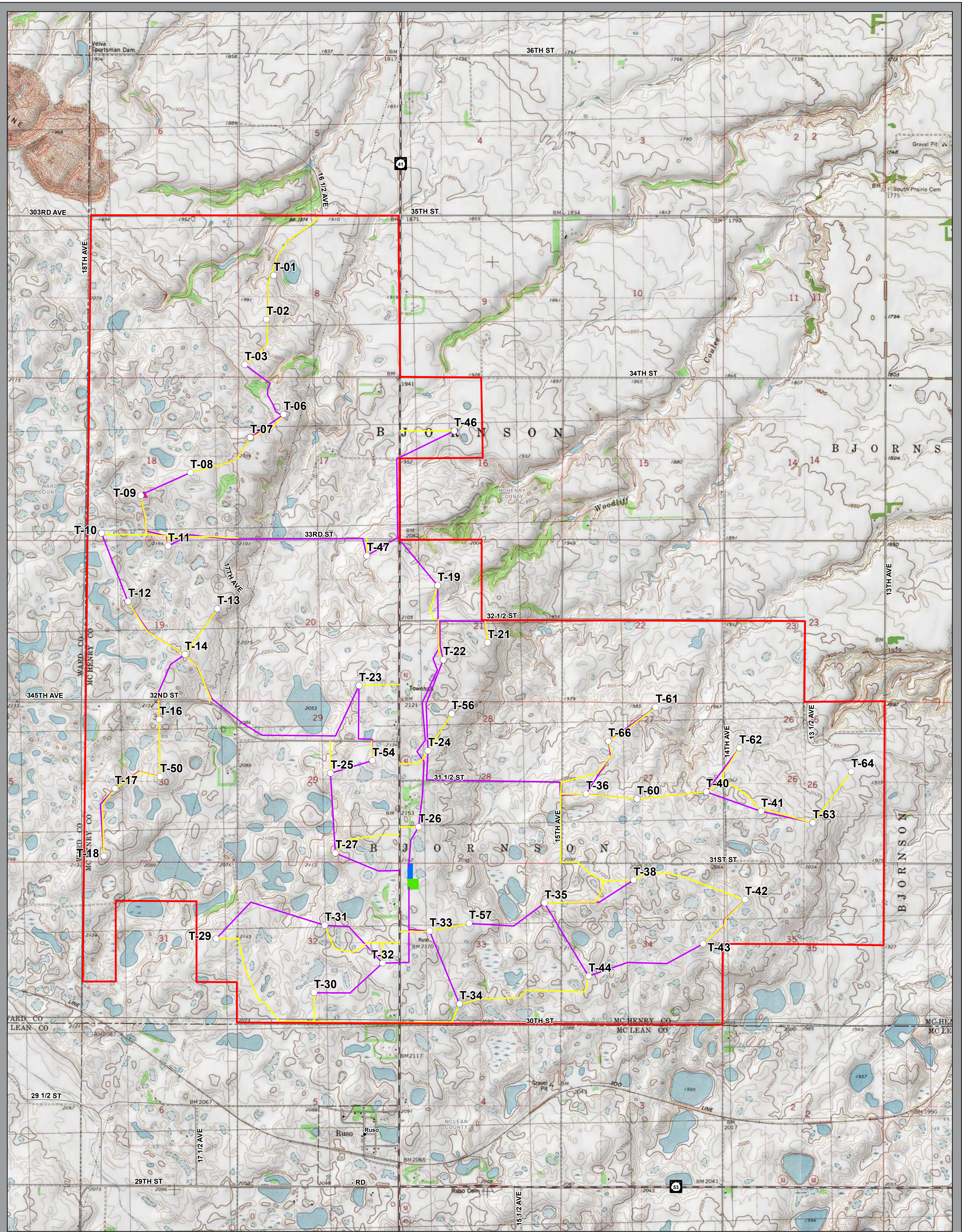
Figure 1. Project Layout
