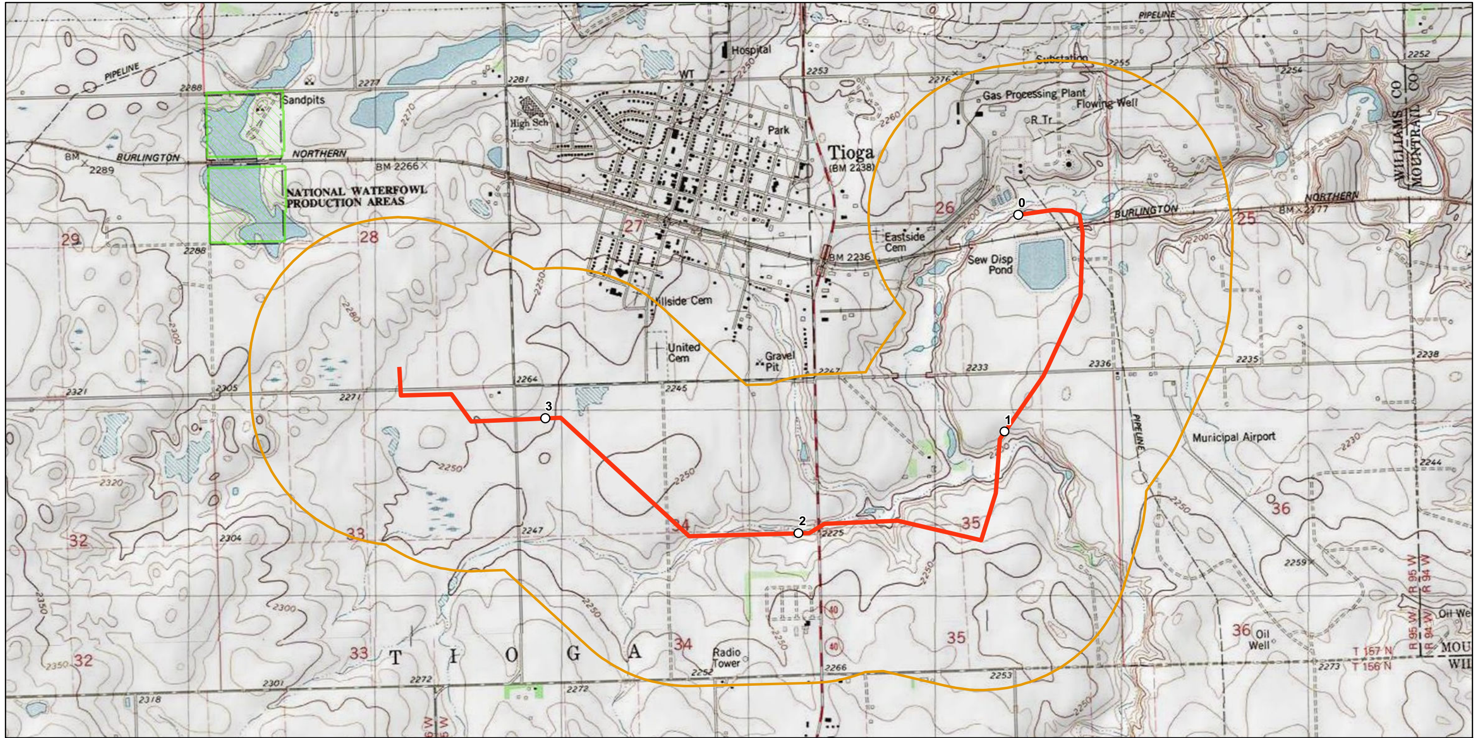
Figure M1 Spur to Tioga Proposed Pipeline
