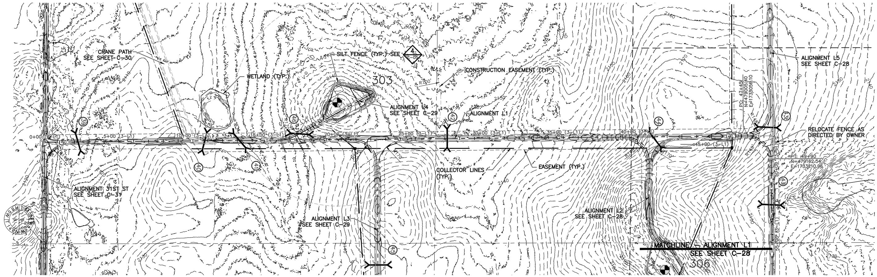
1 PLAN: ALIGNMENT L1 0 200 400 SCALE IN FEET
