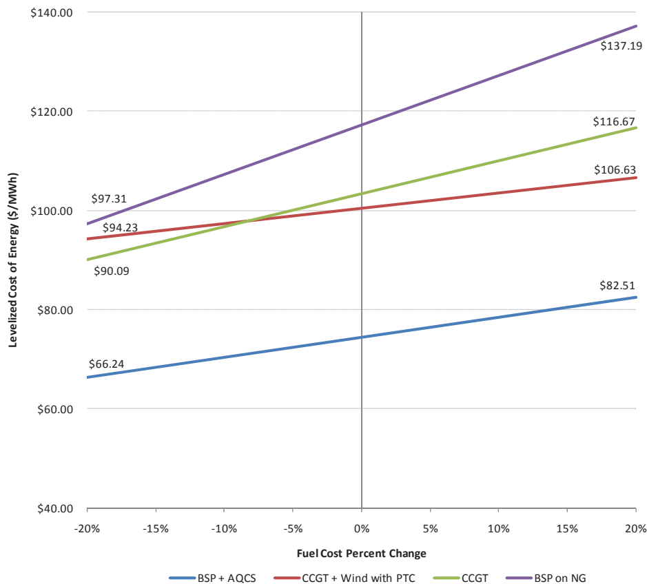
Figure 2 – Fuel Cost Sensivity Levelized Energy Costs
