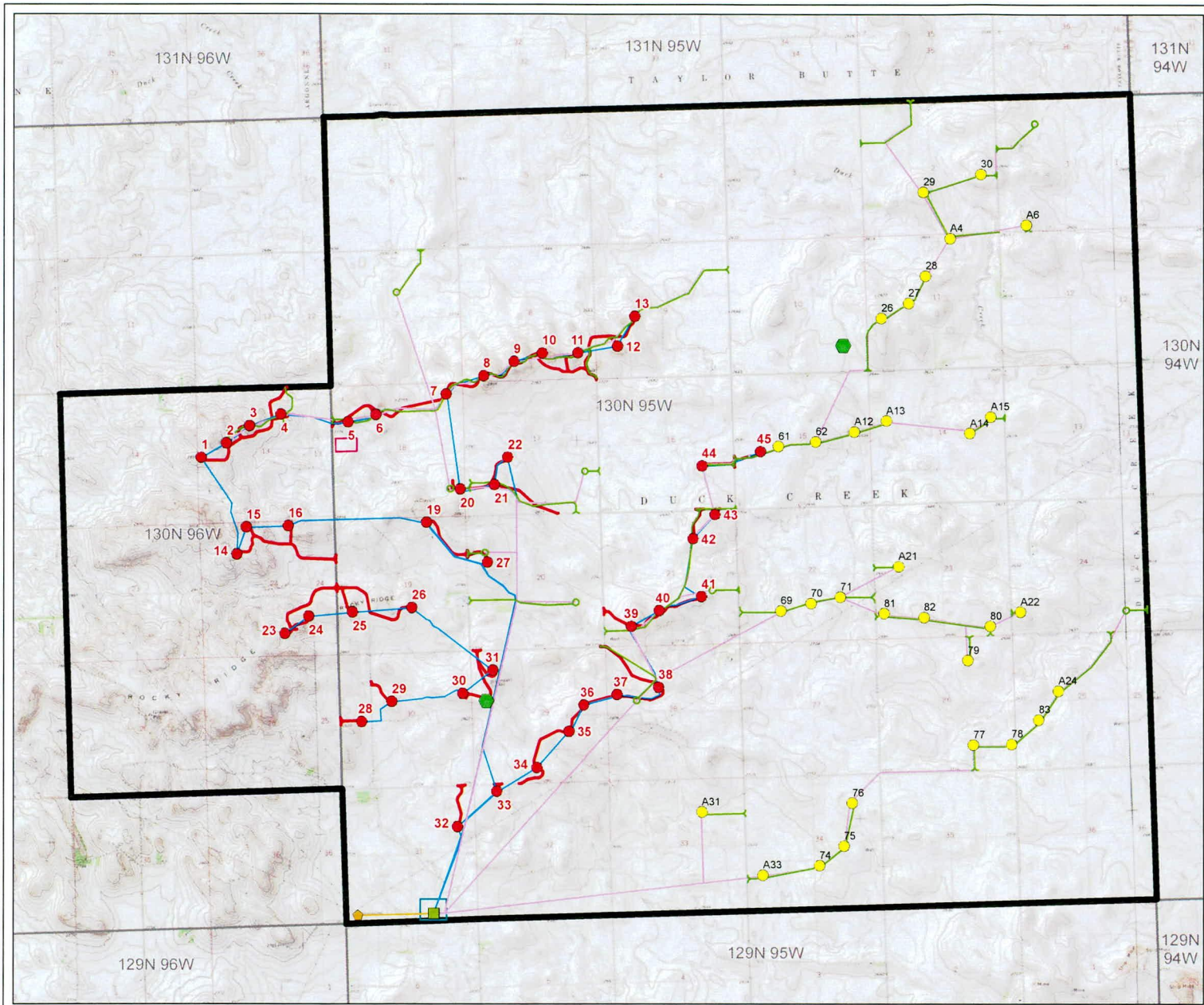
Figure 20 Final Proposed Layout with Optional Phase II Thunder Spirit Wind Energy Project Thunder Spirit Wind, LLC Adams County, North Dakota June 2014
