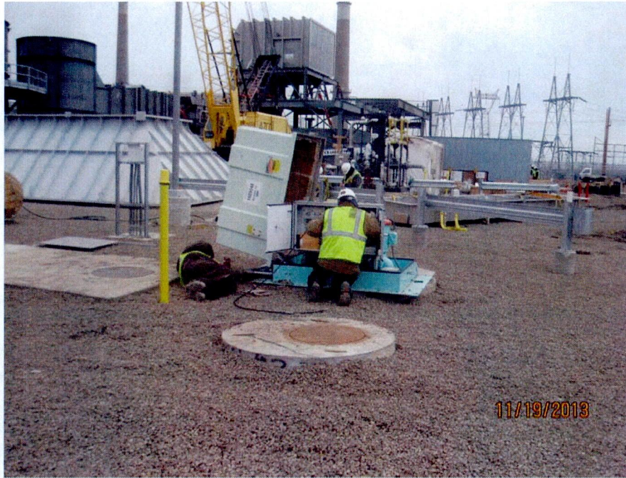
Waste water lift station cable installation (looking E)
