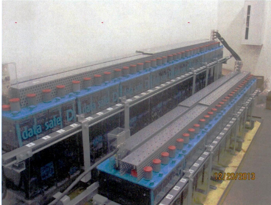
Battery covers and jumper installation (looking NE)
