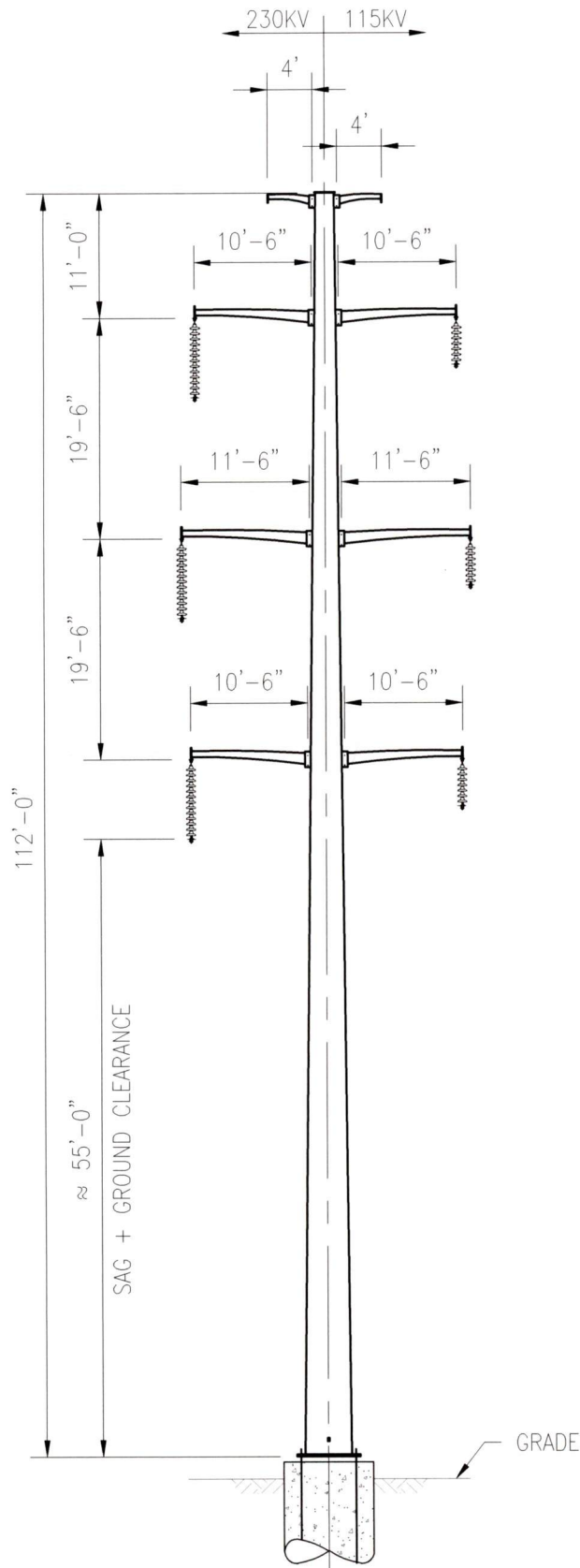
BASIC 230/115KV DOUBLE CIRCUIT STRUCTURE AVERAGE SPAN \approx 800'
