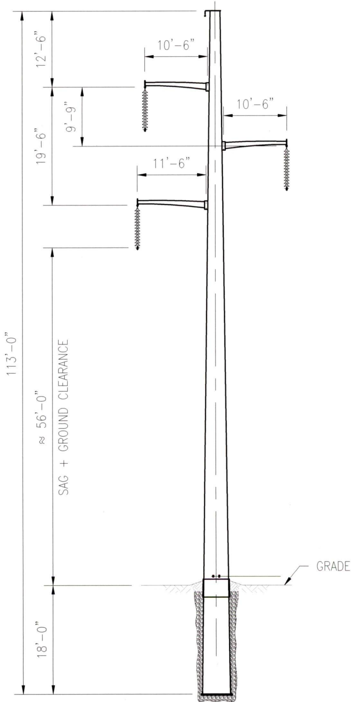
BASIC 230kV SINGLE CIRCUIT STRUCTURE AVERAGE SPAN \approx 800'
