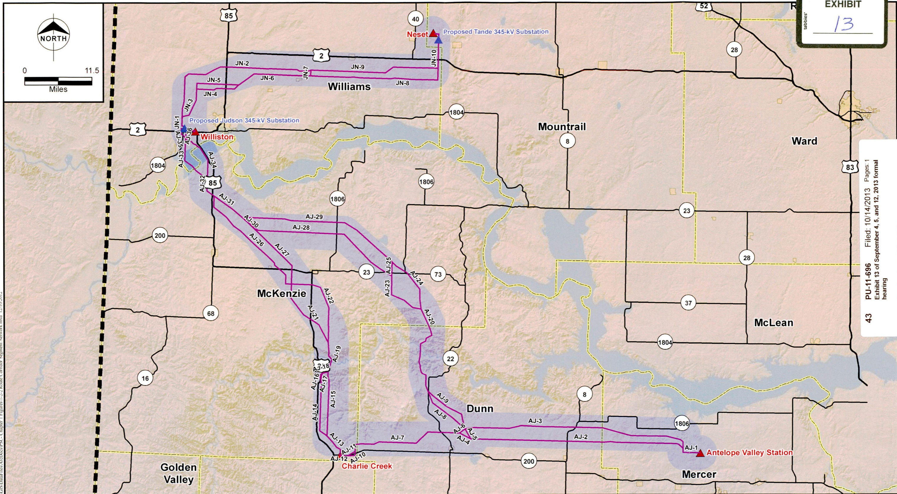
Figure 1.2-2 Basin Electric Power Cooperative Antelope Valley Station to Naset 345-kV Transmission Project Route Corridor Segment Network
