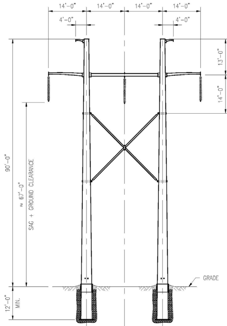
BASIC 345KV SINGLE CIRCUIT H-FRAME STRUCTURE AVERAGE SPAN ≈ 1000'
