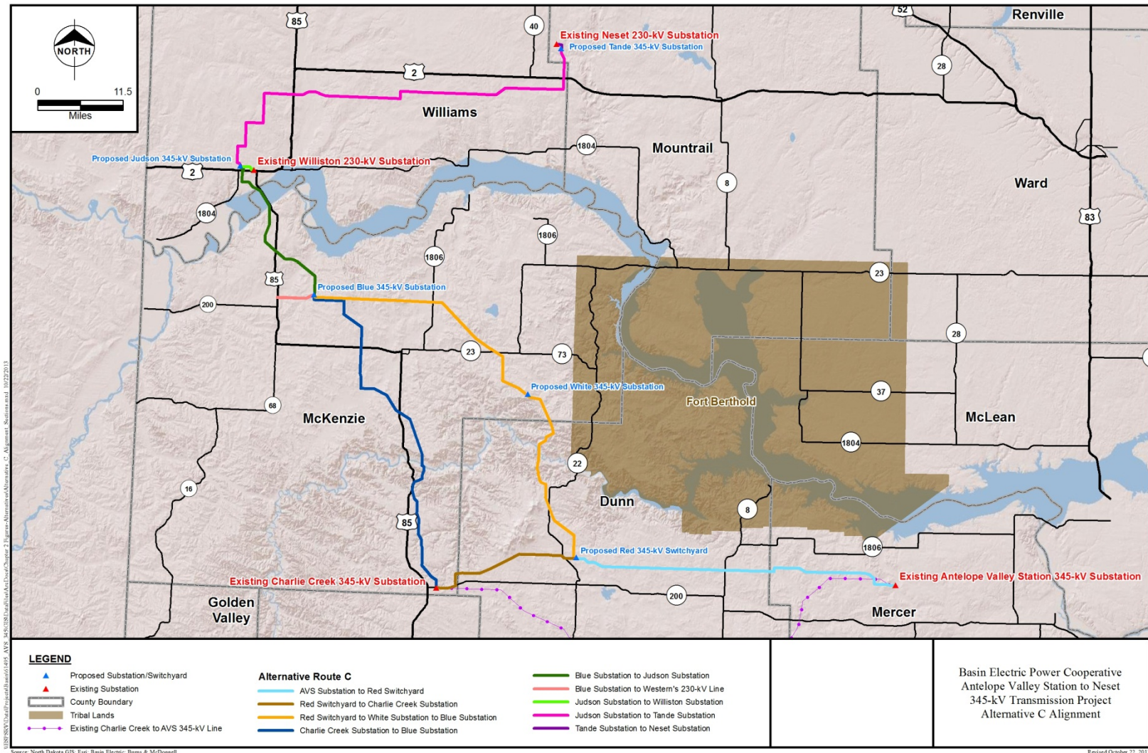
Figure 2-1 Proposed Alternative C for the AVS Transmission Line
