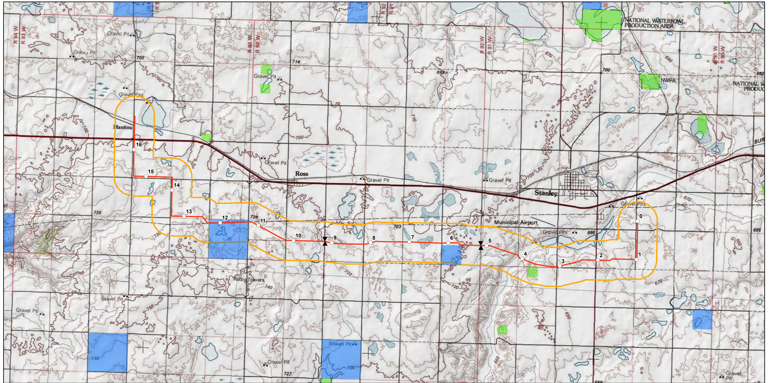
Figure M1 Nelson to Ross Proposed Pipeline Overview Map
