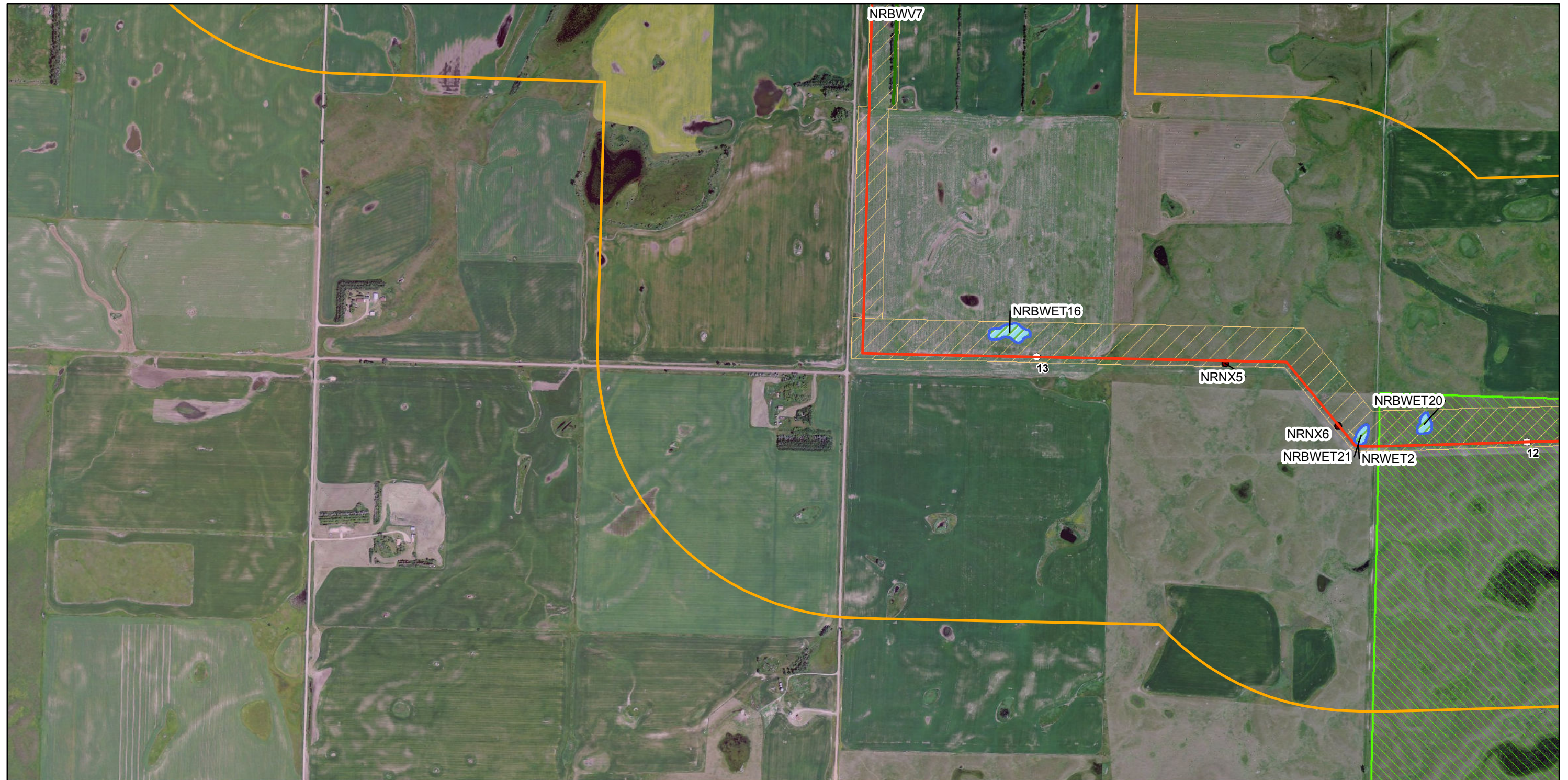
Figure SC-07 Nelson to Ross Proposed Pipeline Siting Criteria
