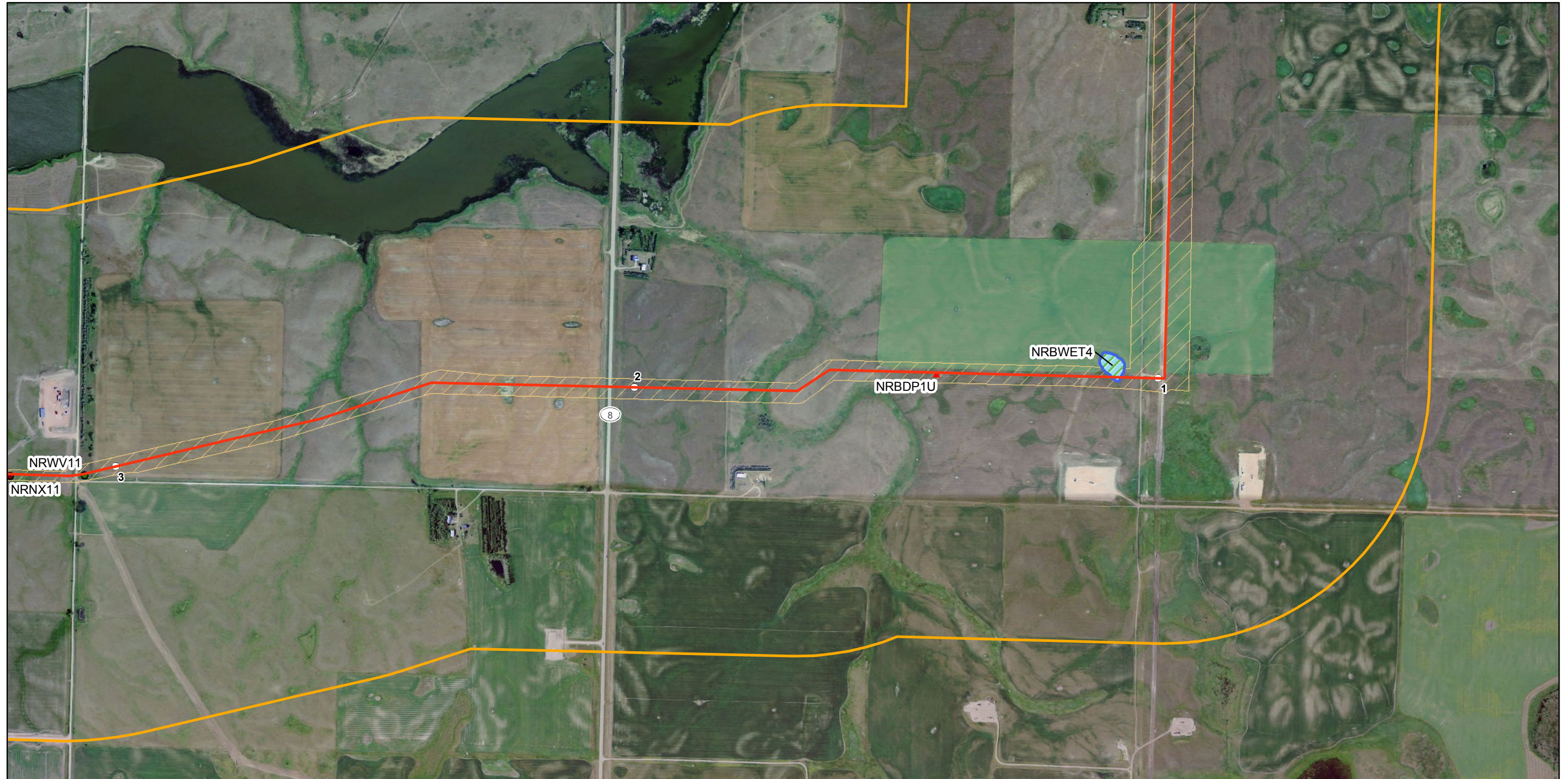
Figure SC-02 Nelson to Ross Proposed Pipeline Siting Criteria
