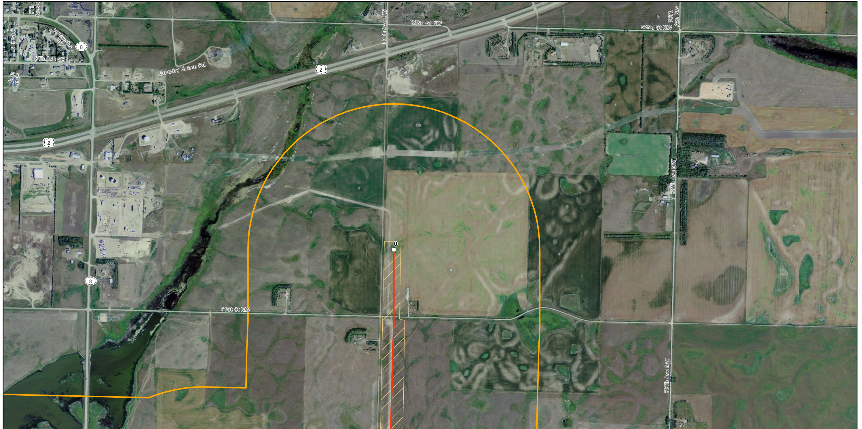
Figure SC-CR-01 Nelson to Ross Proposed Pipeline Siting Criteria
