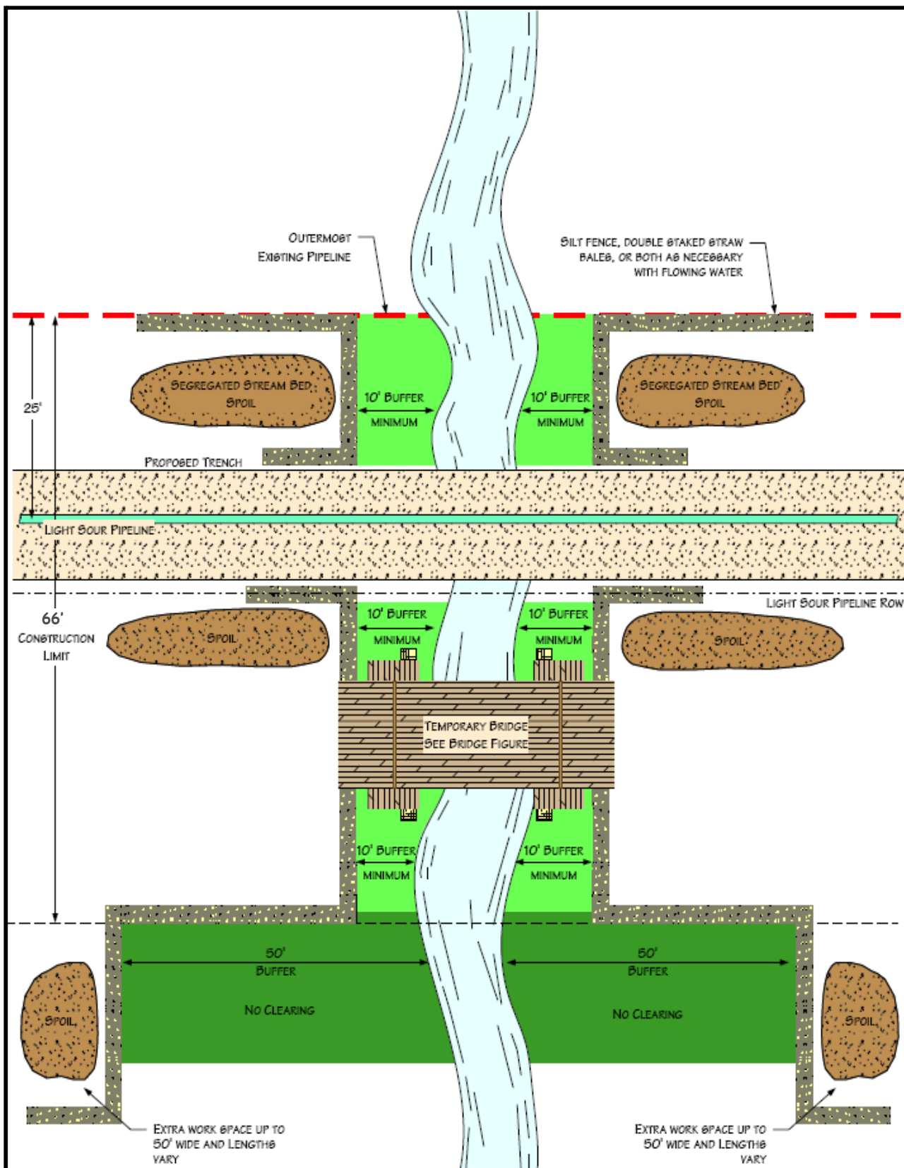
Figure 6.2.1 – Typical Waterbody Crossing Wet Trench Method 6-inch Natural Gas Residue Pipeline January 2013
