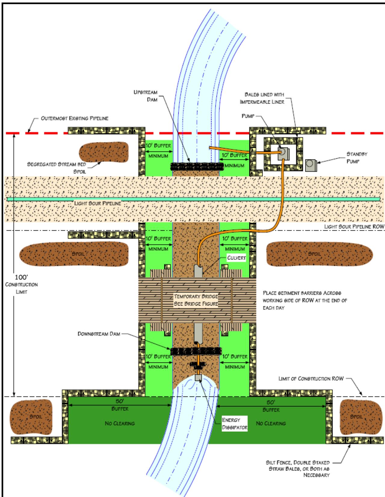
Figure 6.2.2 – Typical Waterbody Crossing Dam and Pump Method 6-inch Natural Gas Residue Pipeline January 2013
