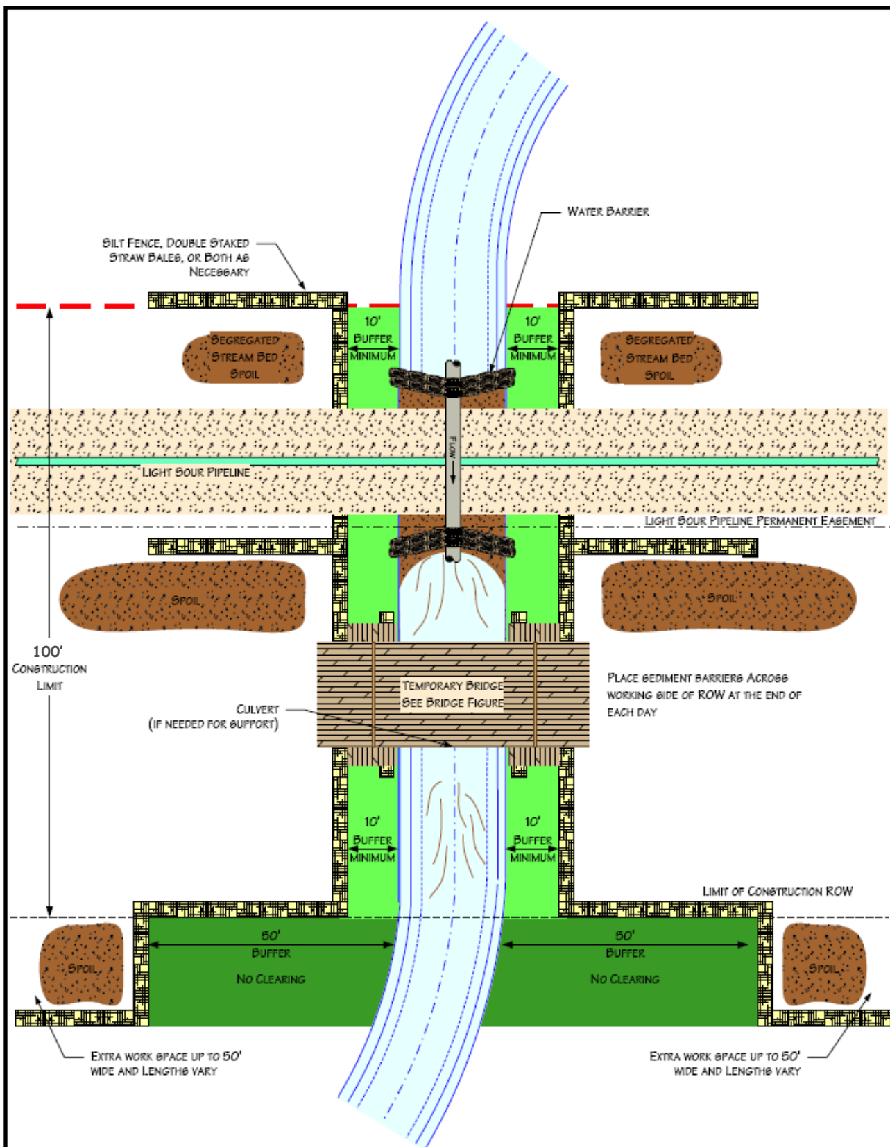
Figure 6.2.3 –Typical Waterbody Crossing Flume Method 6-inch Natural Gas Residue Pipeline January 2013
