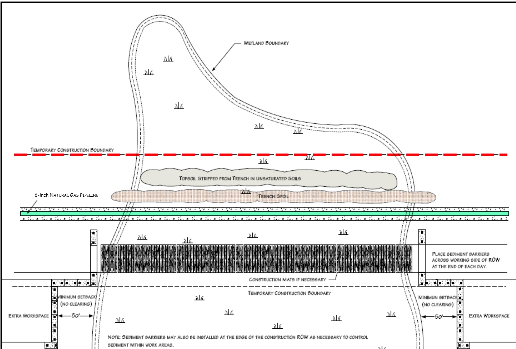
Figure 6.3.1 – Typical Wetland Crossing Method 6-inch Natural Gas Residue Pipeline January 2013
