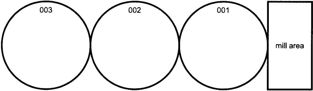
SECTION A 3 concrete silos 75' diameter x 150' depth
