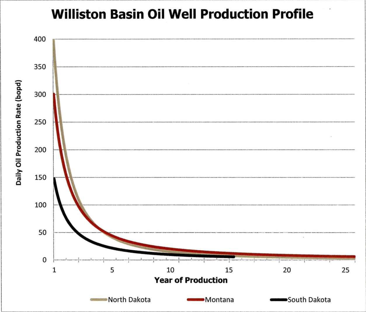
Figure 25: Williston Basin Oil Well Production Profiles
