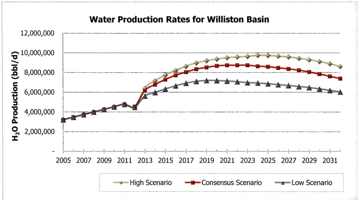
Figure 19: Water Production Rates for Williston Basin Source: University of North Dakota
