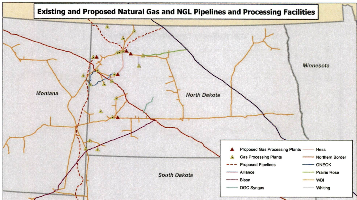
Figure 28: Existing and Proposed Natural Gas and NGL Pipelines and Processing Facilities
