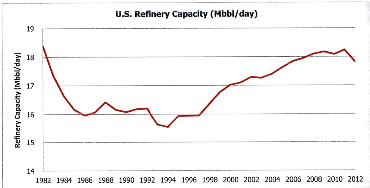
Figure 29: U.S. Refinery Capacity (Million Barrels per Day) Source: U.S. Energy Information Administration
