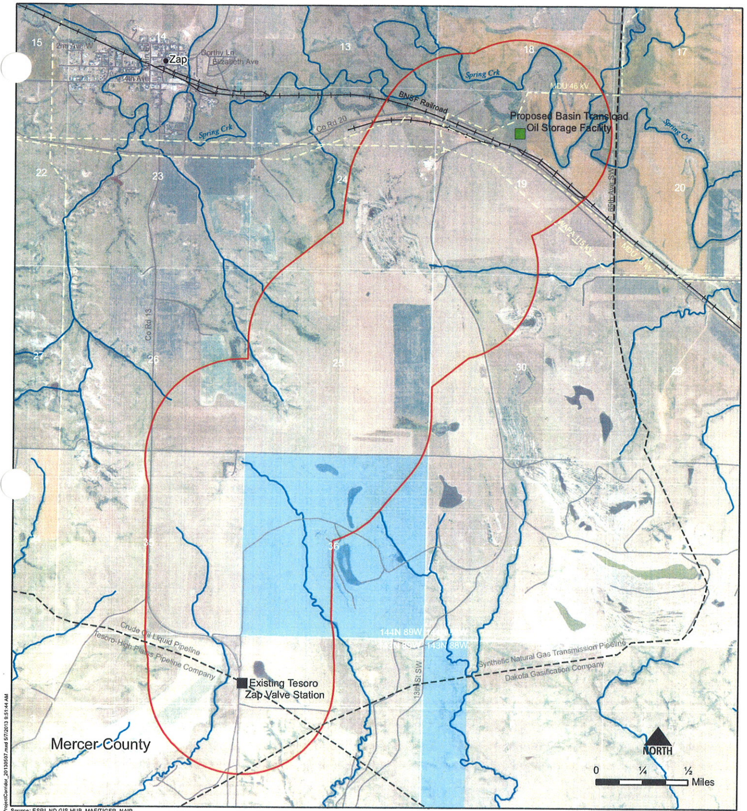
Figure 1-1 THPP Beulah Lateral Pipeline Project Corridor
