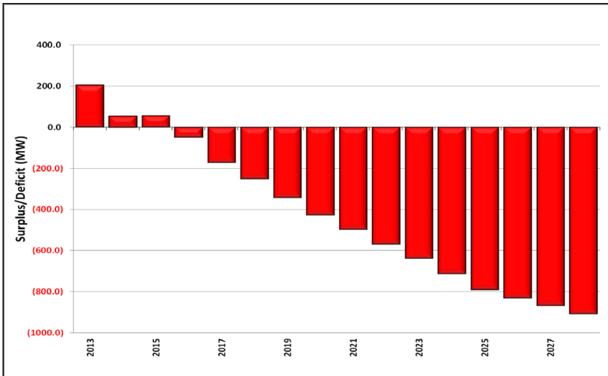
Figure 3. IS (WAUE) System Surplus Capacity
