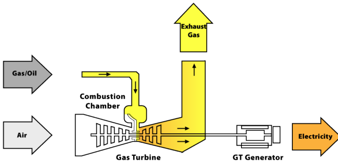
Figure 4-1: Simple Cycle Unit Process Flow Diagram
