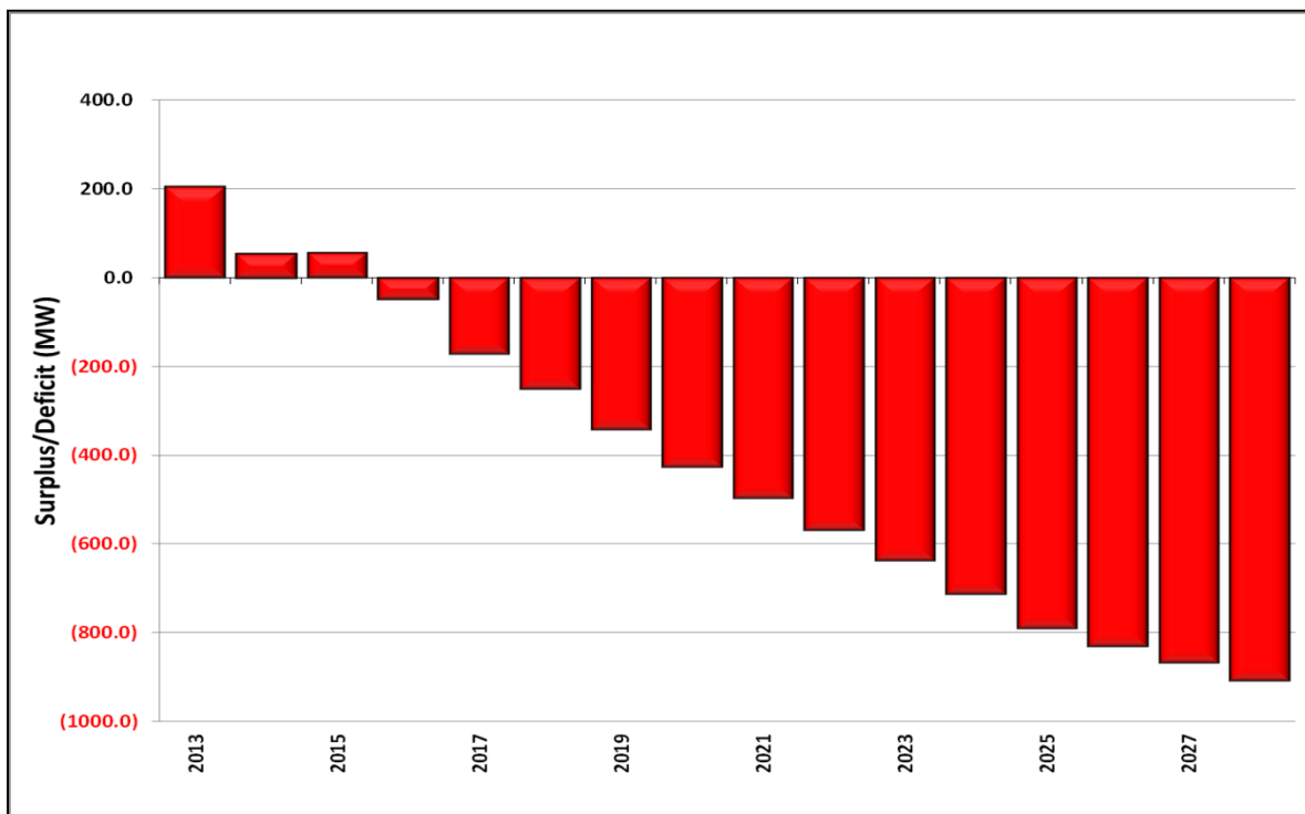
Figure 3-3: IS (WAUE) System Surplus/Deficit
