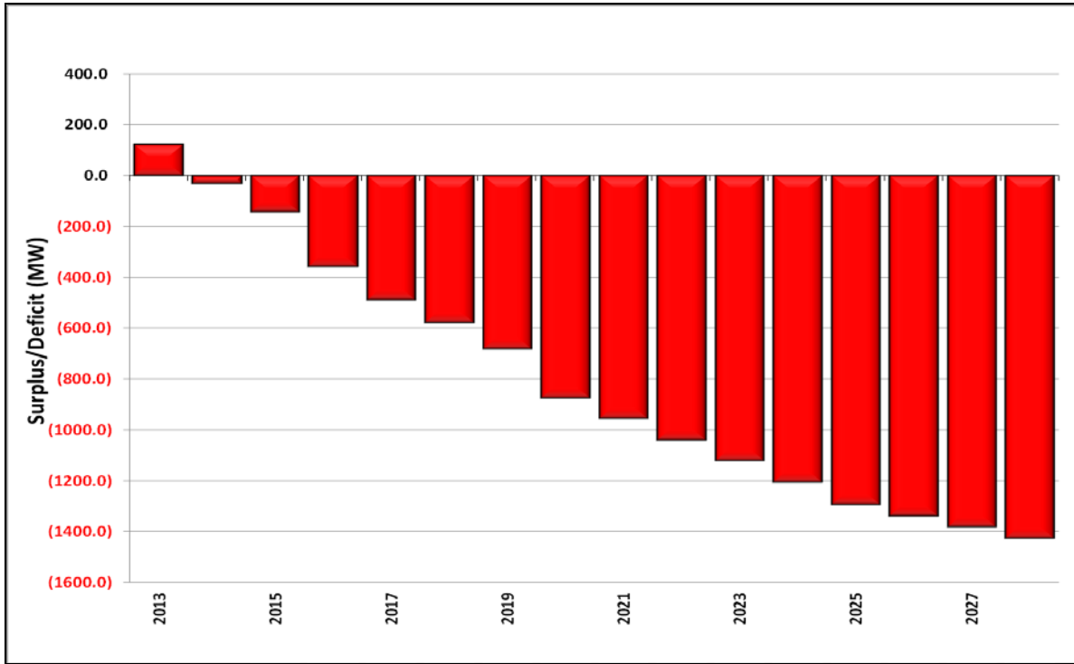
Figure 2. East System Summer Surplus
