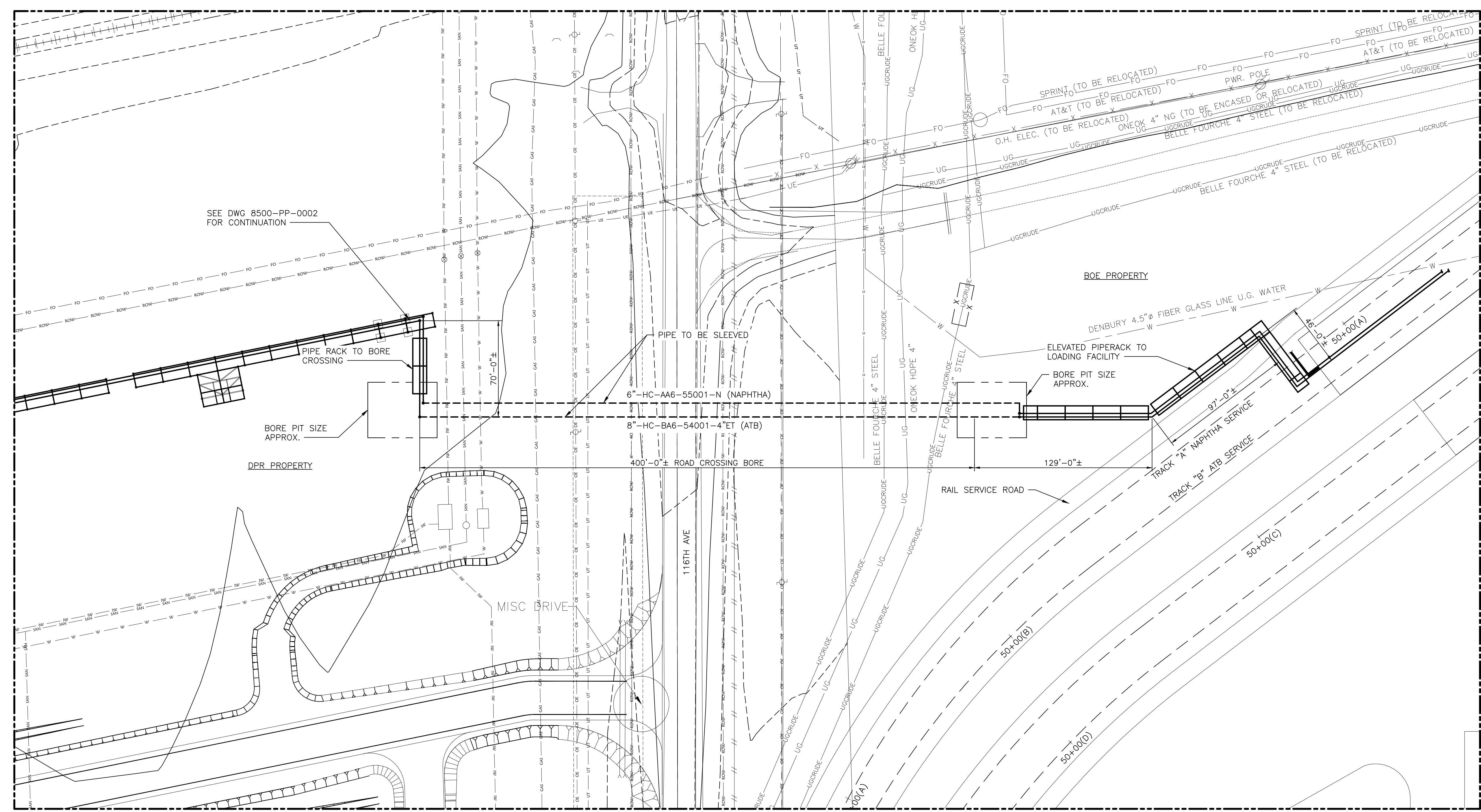
DPR TO BOE INTERFACE – PLAN VIEW 1"=40'
